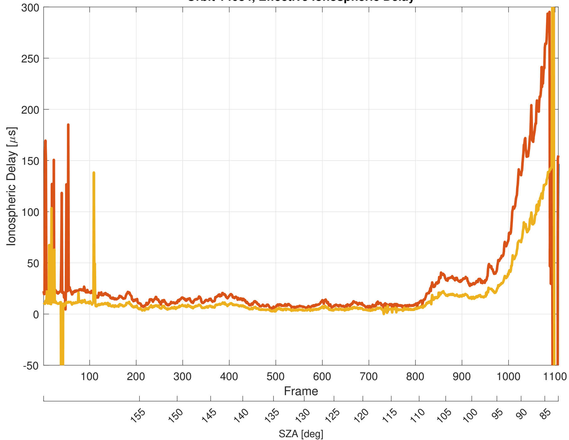
Orbit 14084, Effective Ionospheric Delay
