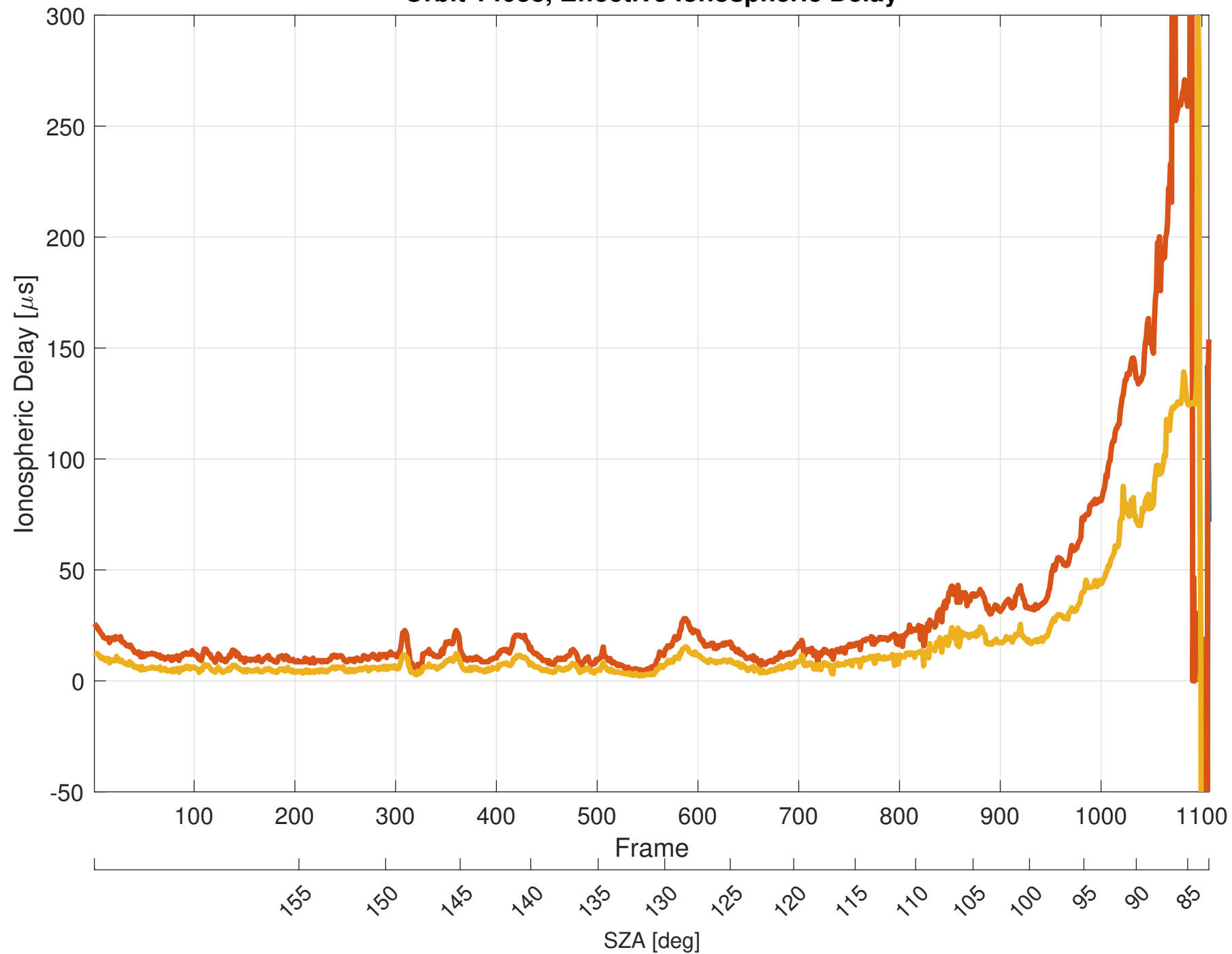
Orbit 14088, Effective Ionospheric Delay
