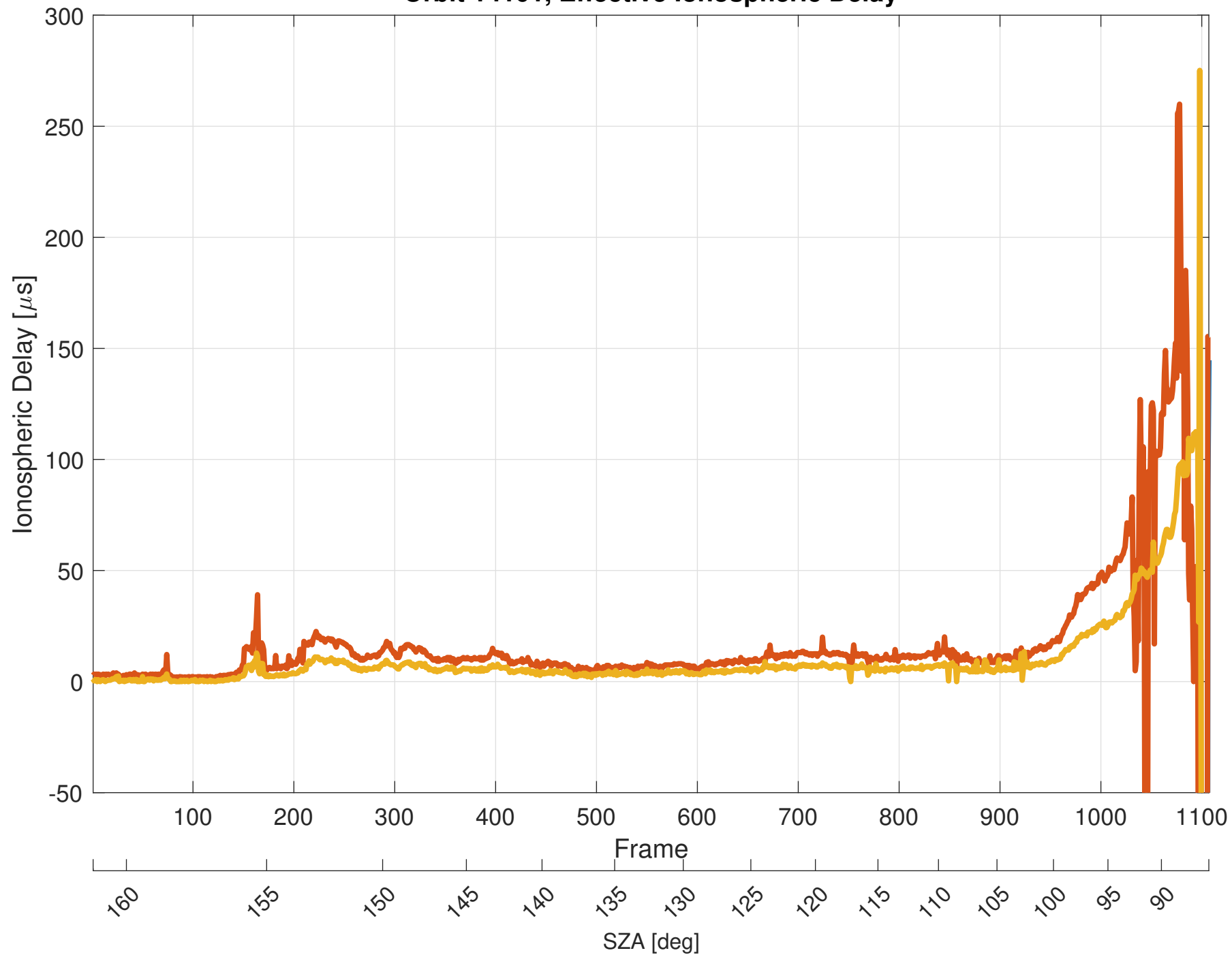
Orbit 14101, Effective Ionospheric Delay
