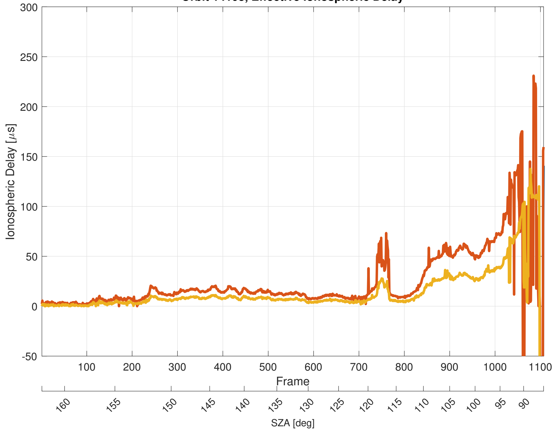
Orbit 14103, Effective Ionospheric Delay
