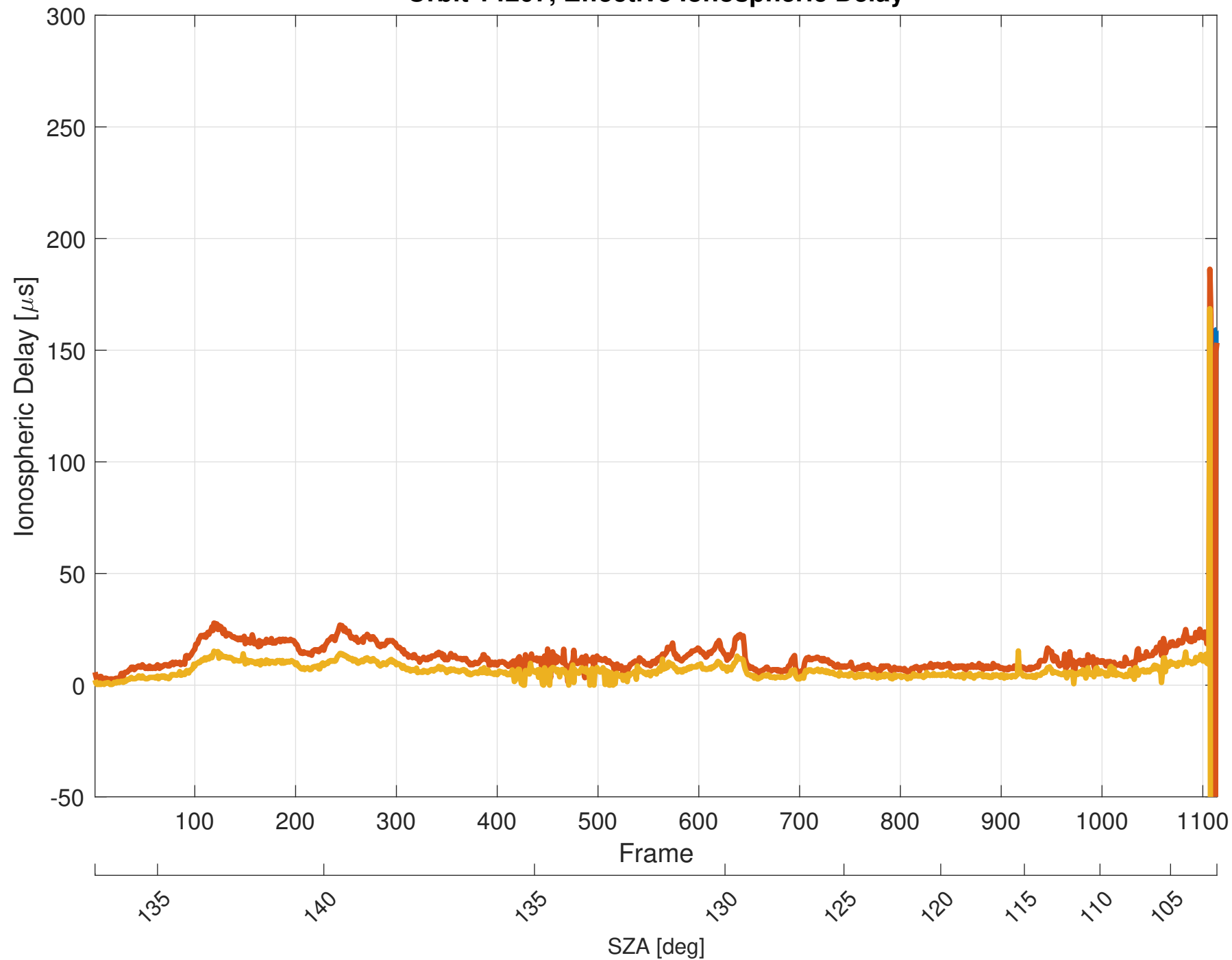
Orbit 14207, Effective Ionospheric Delay
