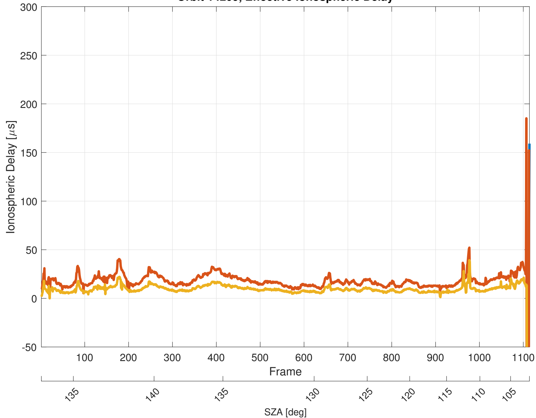
Orbit 14209, Effective Ionospheric Delay
