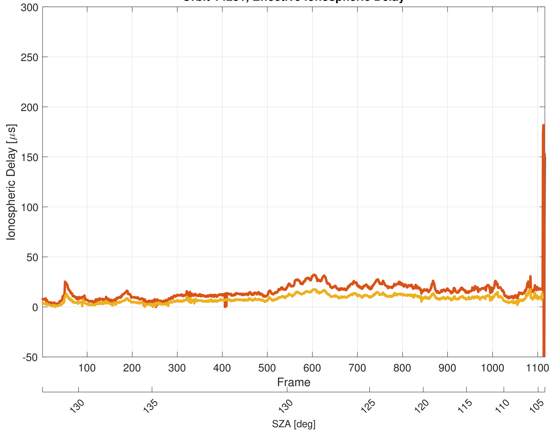
Orbit 14231, Effective Ionospheric Delay
