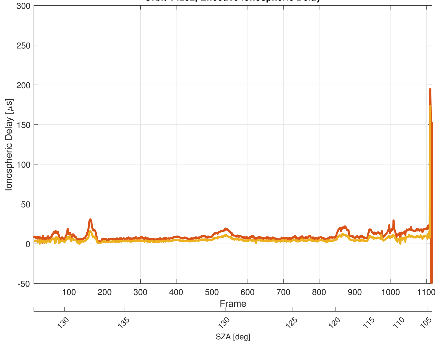
Orbit 14232, Effective Ionospheric Delay
