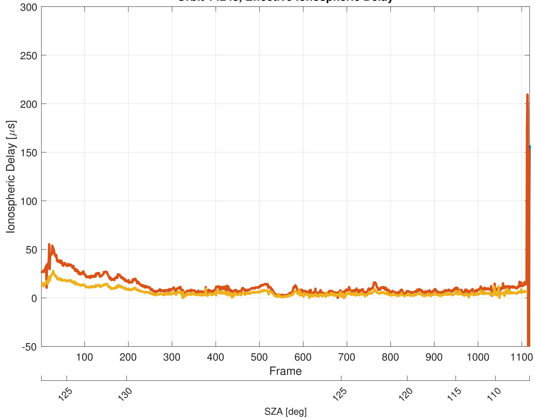
Orbit 14248, Effective Ionospheric Delay
