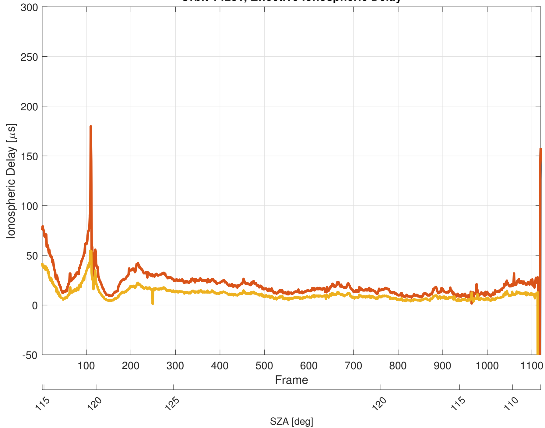
Orbit 14281, Effective Ionospheric Delay
