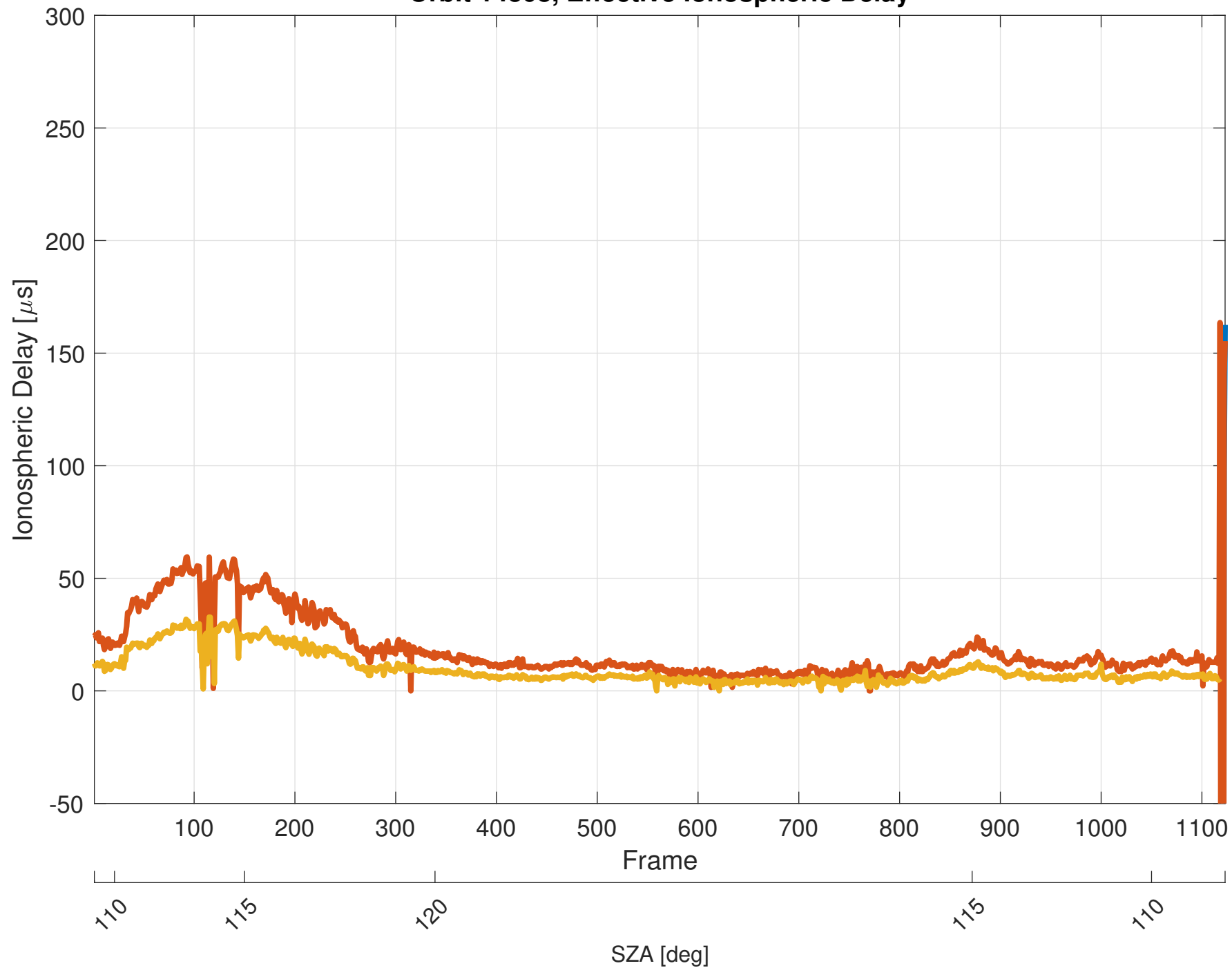
Orbit 14308, Effective Ionospheric Delay
