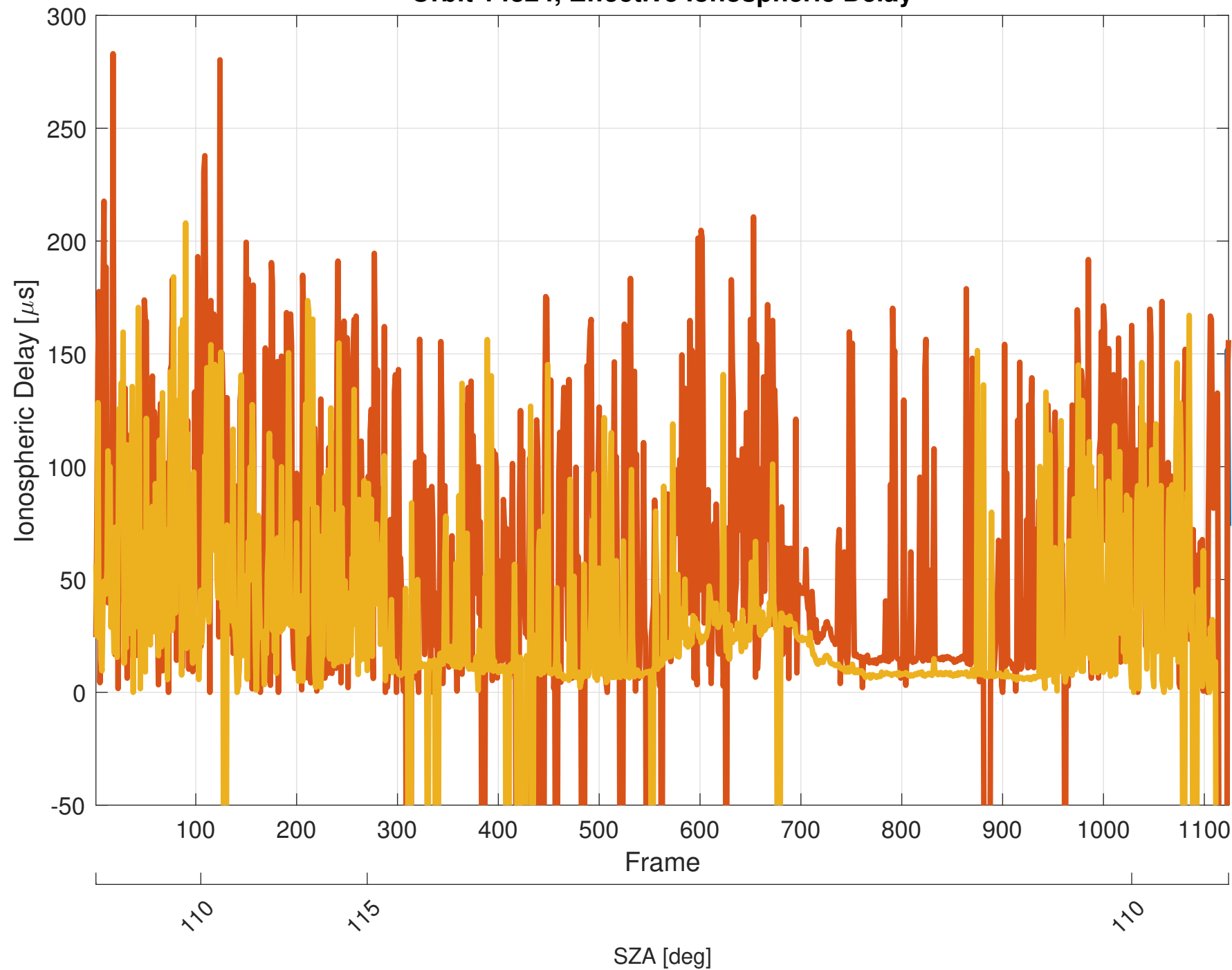
Orbit 14324, Effective Ionospheric Delay
