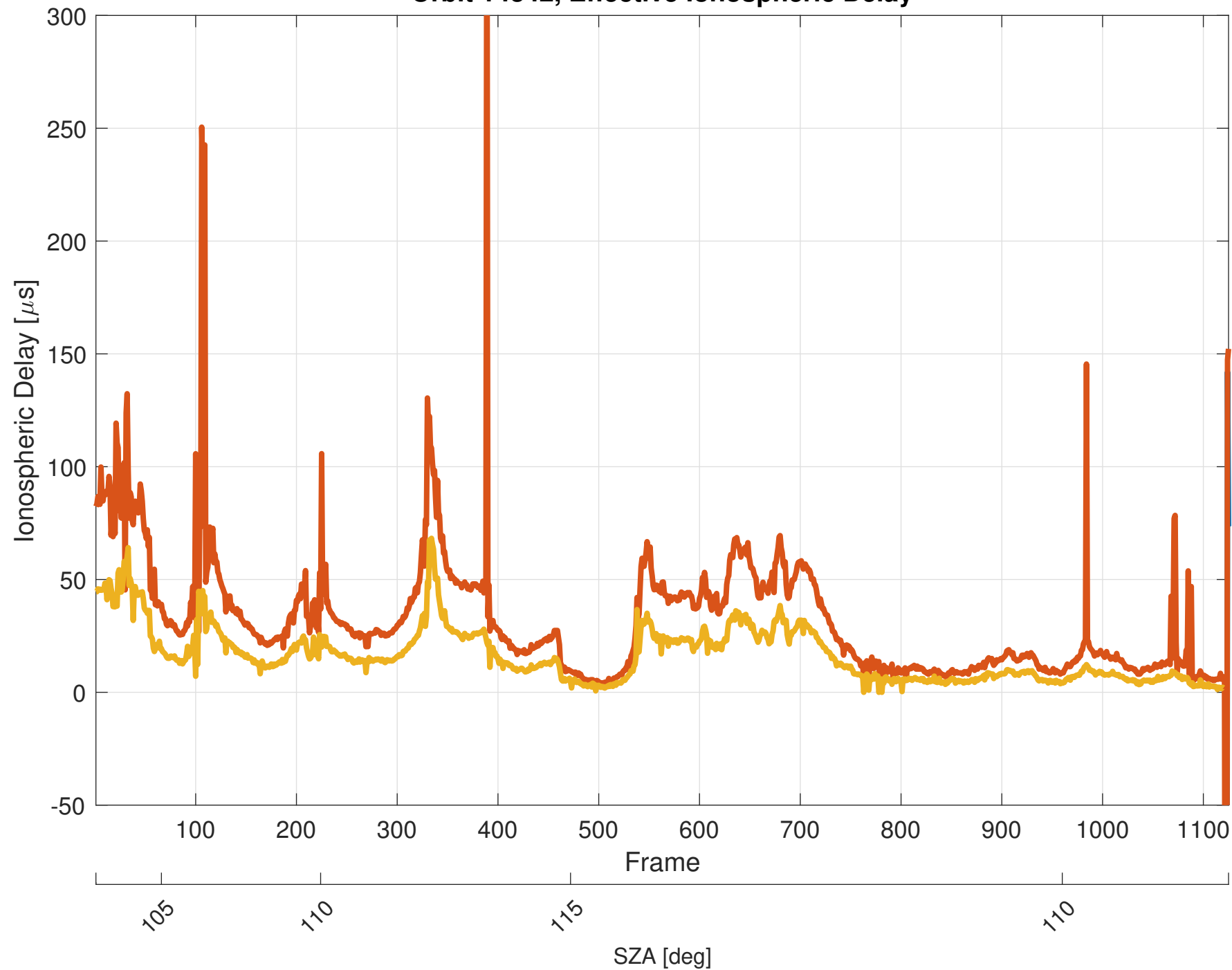
Orbit 14342, Effective Ionospheric Delay
