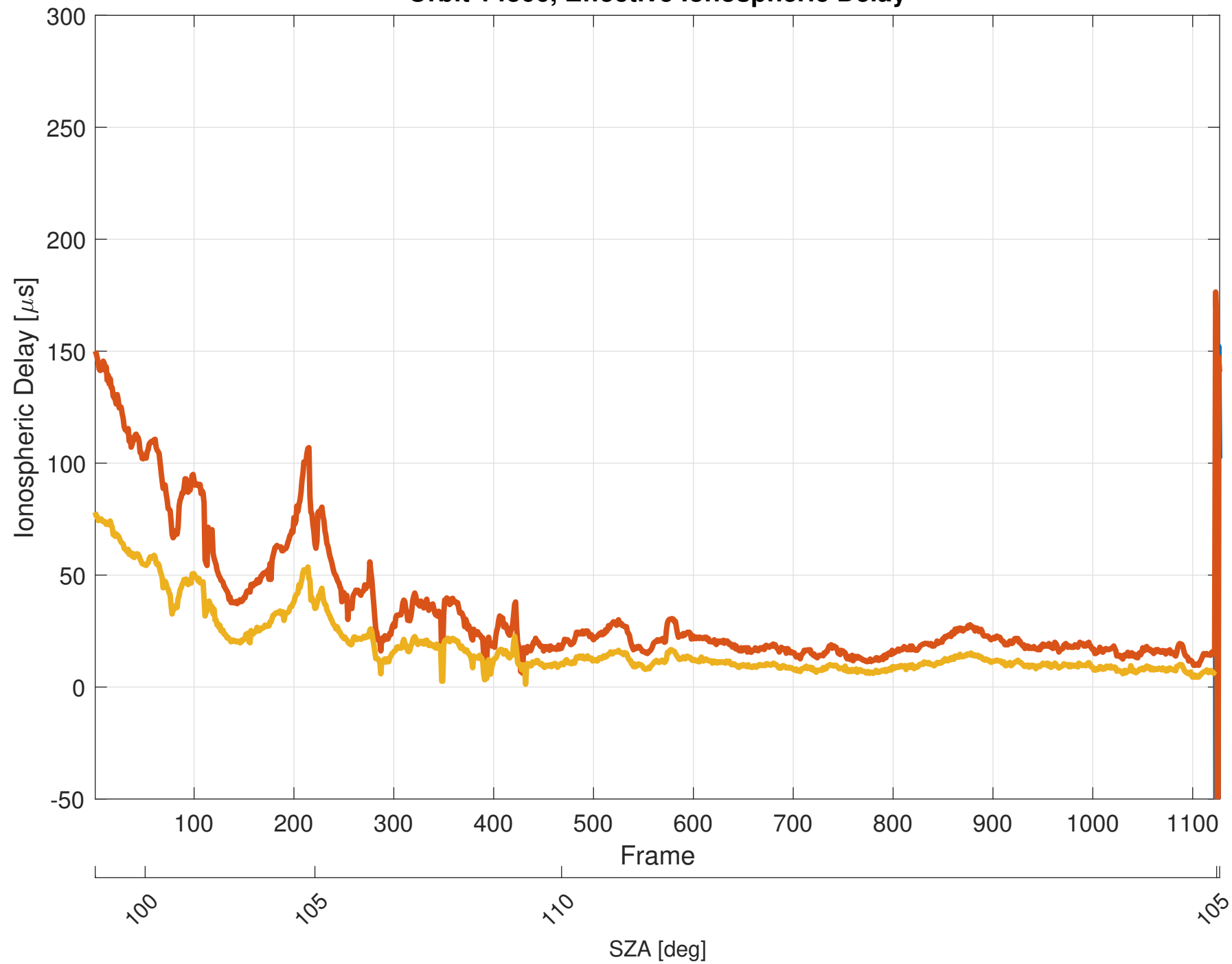
Orbit 14366, Effective Ionospheric Delay
