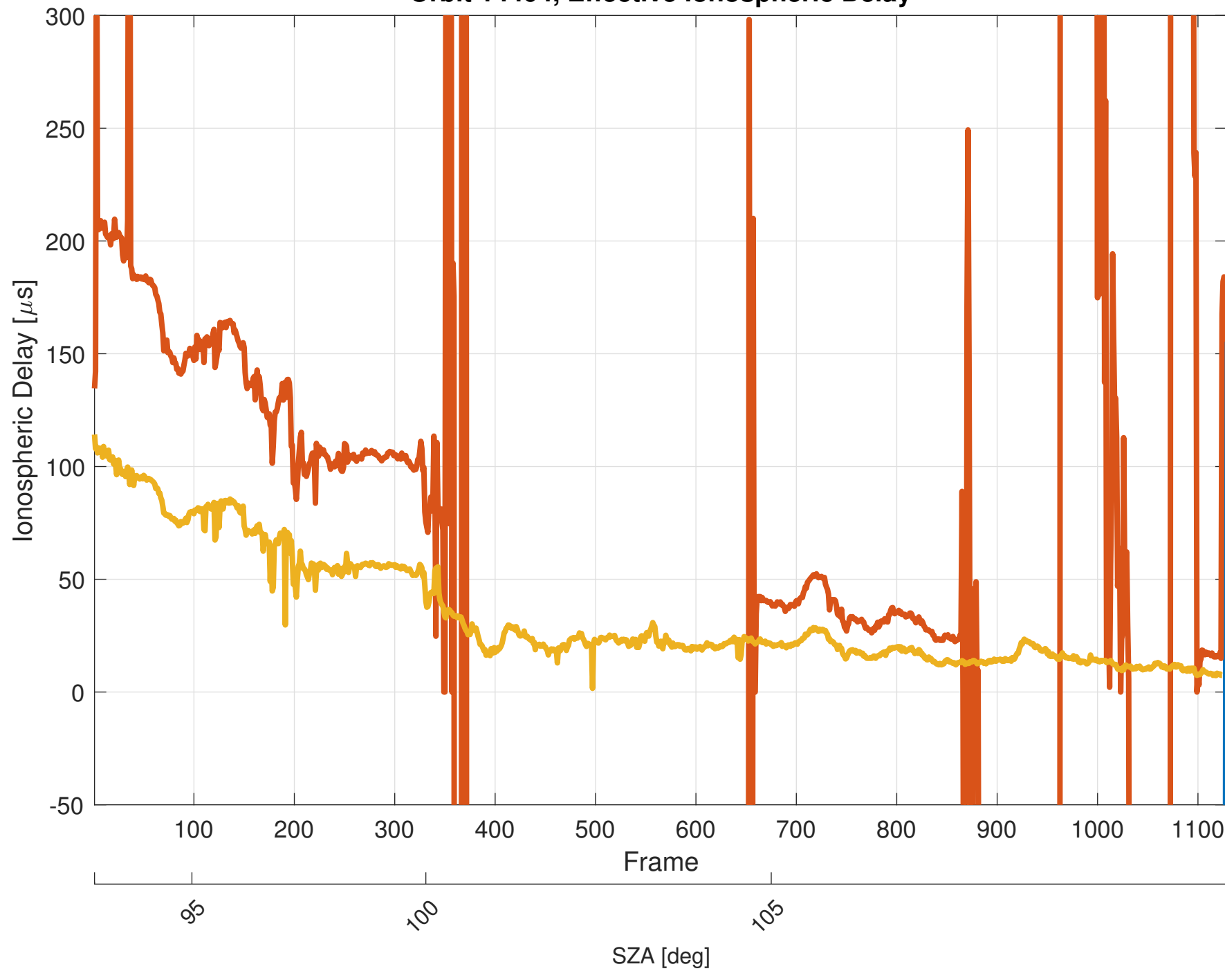
Orbit 14404, Effective Ionospheric Delay
