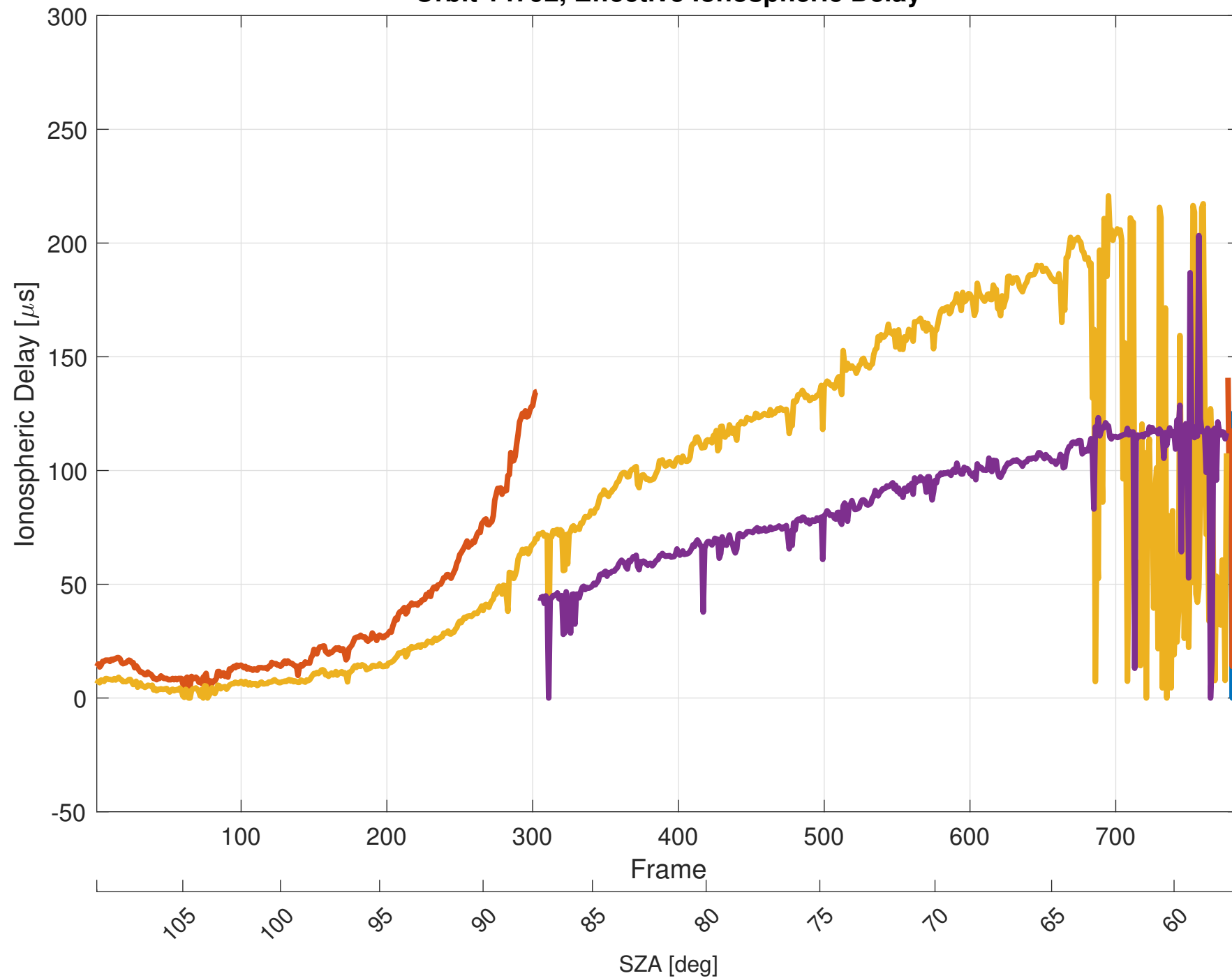
Orbit 14792, Effective Ionospheric Delay
