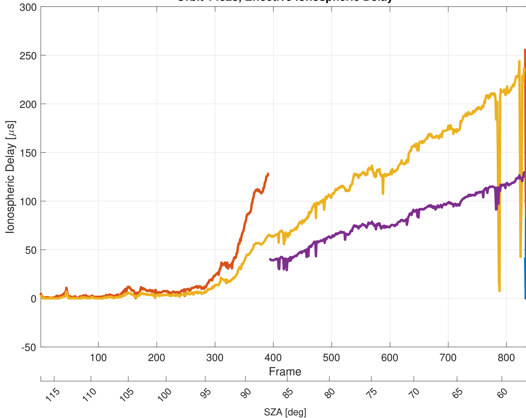
Orbit 14828, Effective Ionospheric Delay
