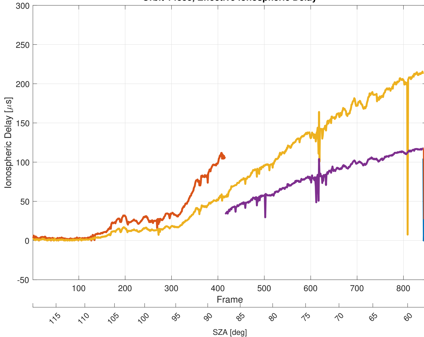
Orbit 14838, Effective Ionospheric Delay
