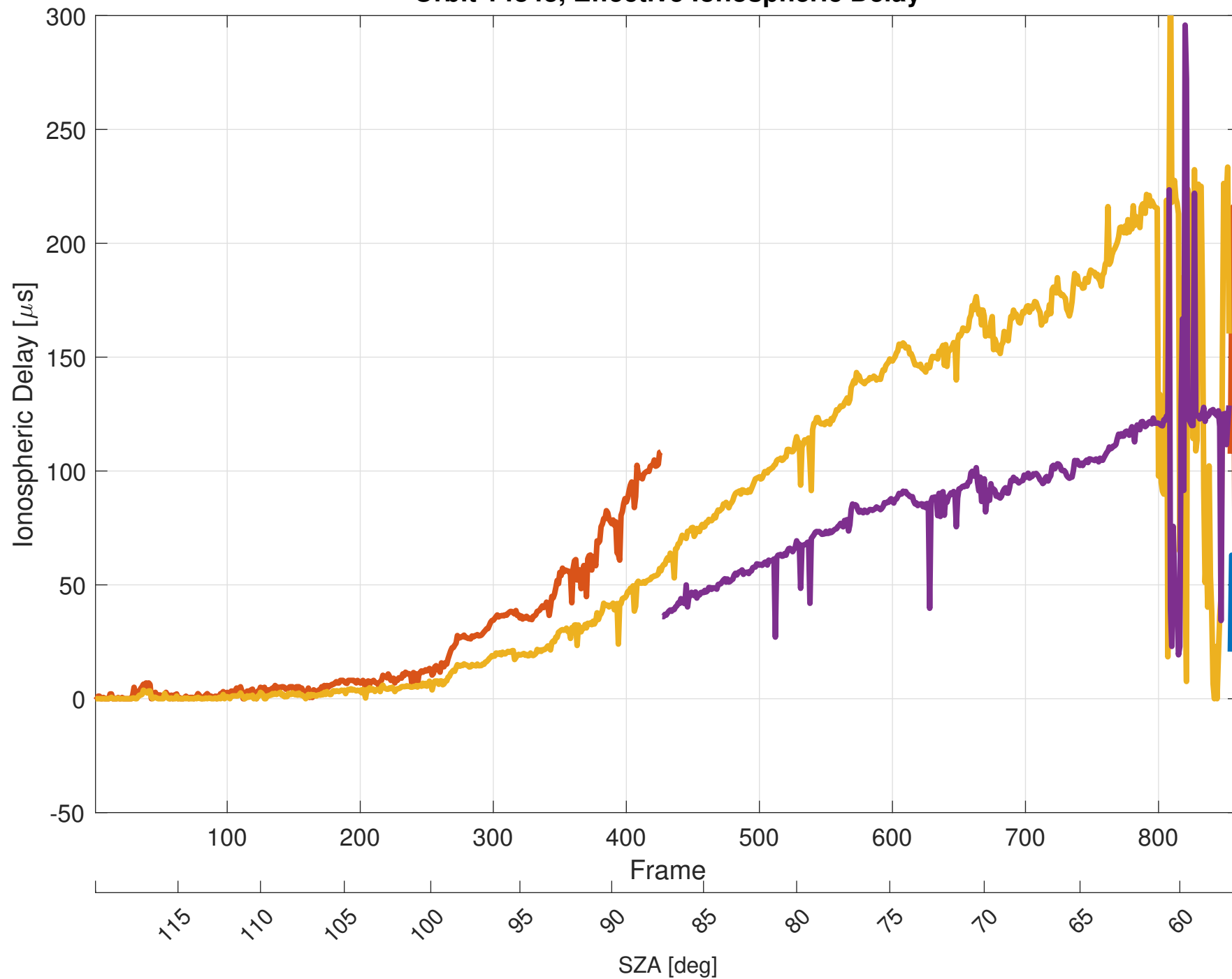
Orbit 14843, Effective Ionospheric Delay
