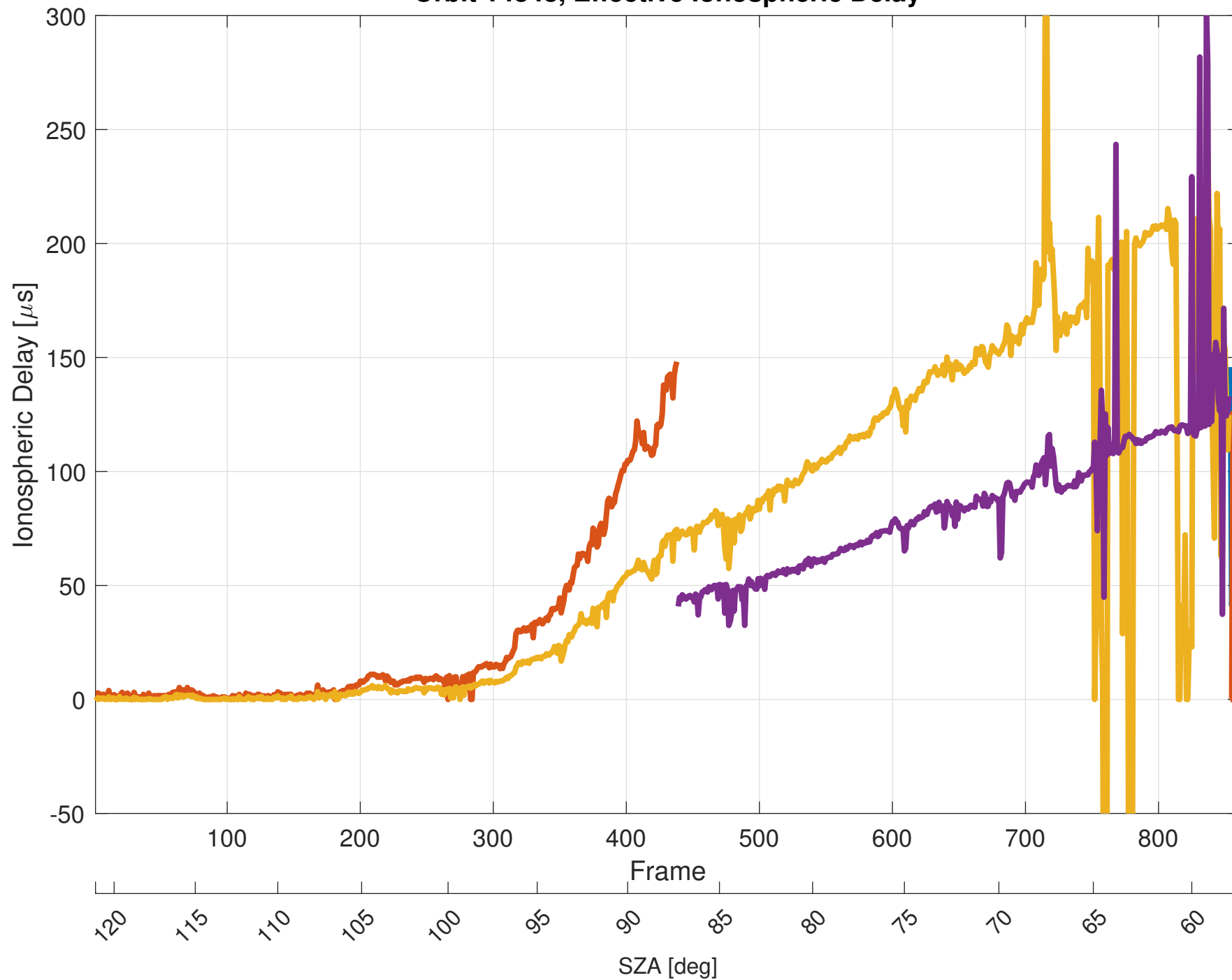
Orbit 14848, Effective Ionospheric Delay
