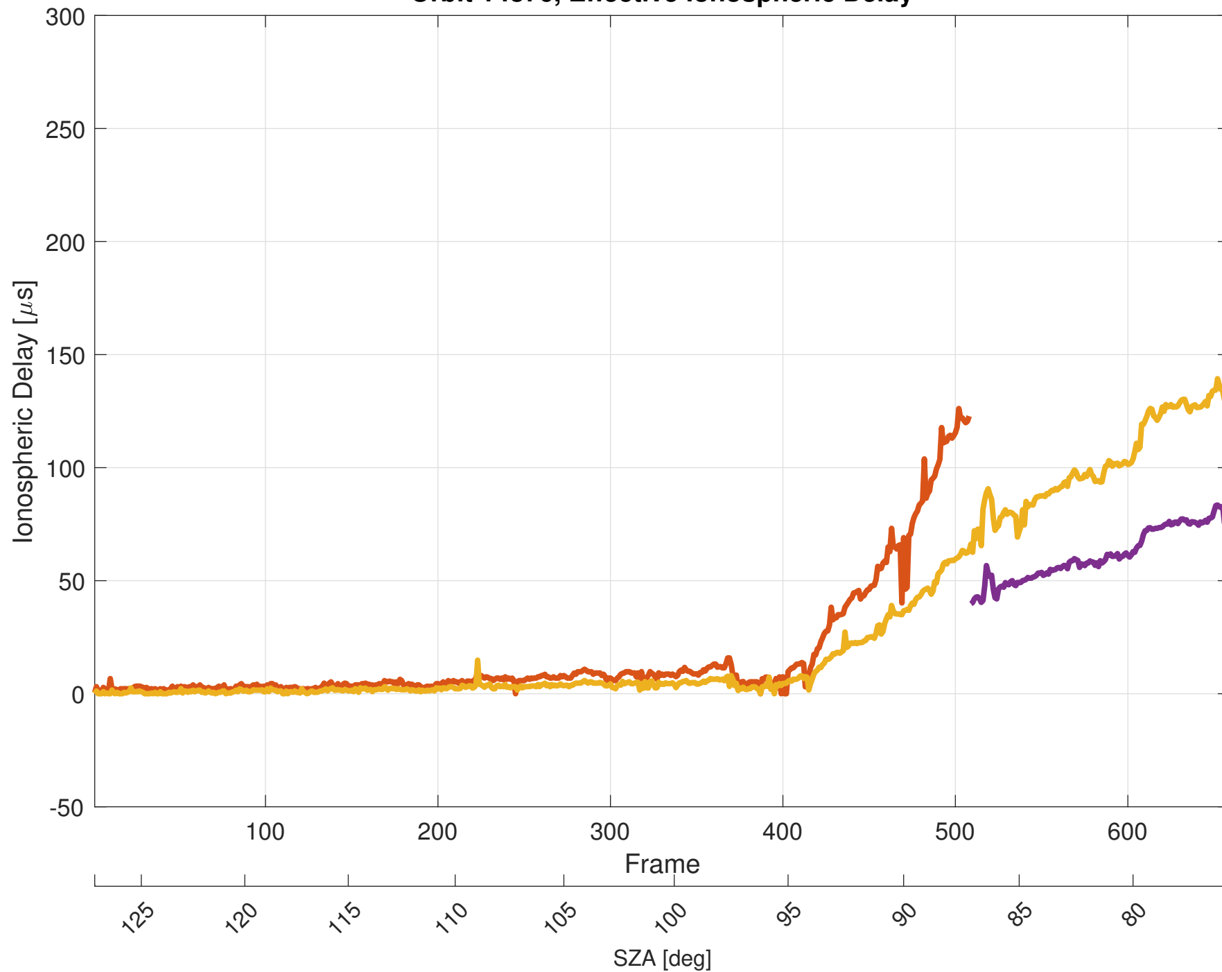
Orbit 14876, Effective Ionospheric Delay
