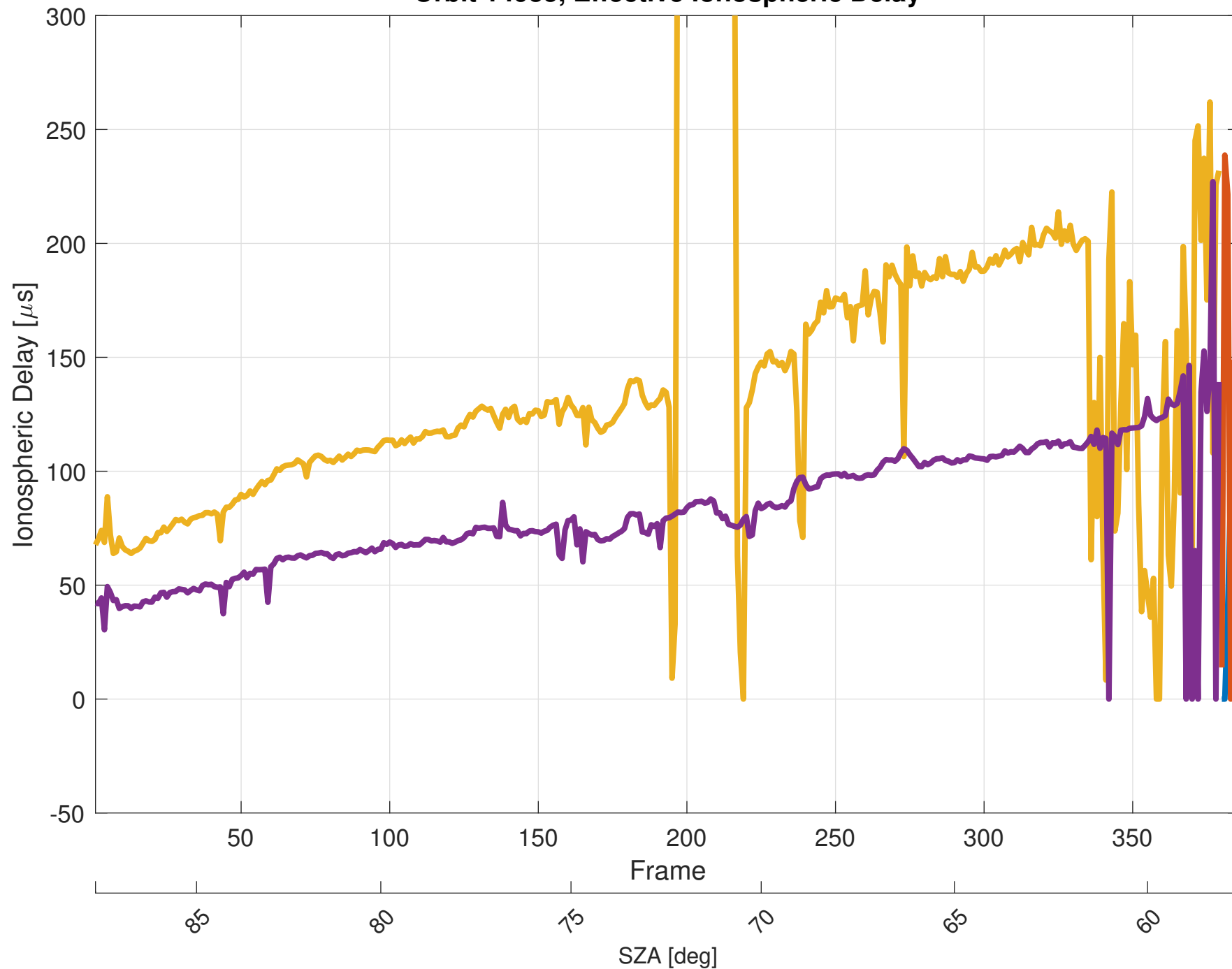
Orbit 14935, Effective Ionospheric Delay
