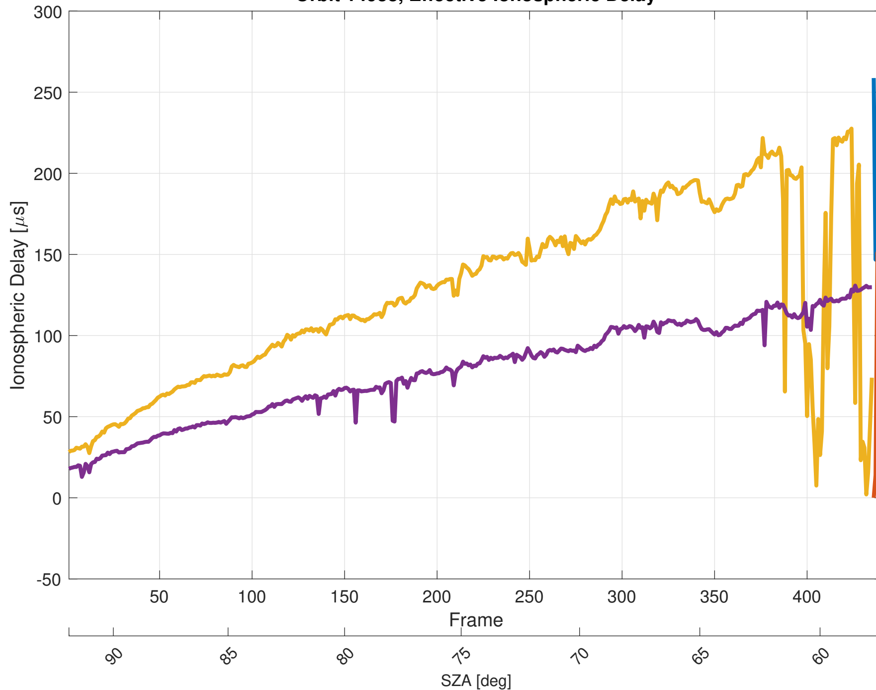
Orbit 14938, Effective Ionospheric Delay
