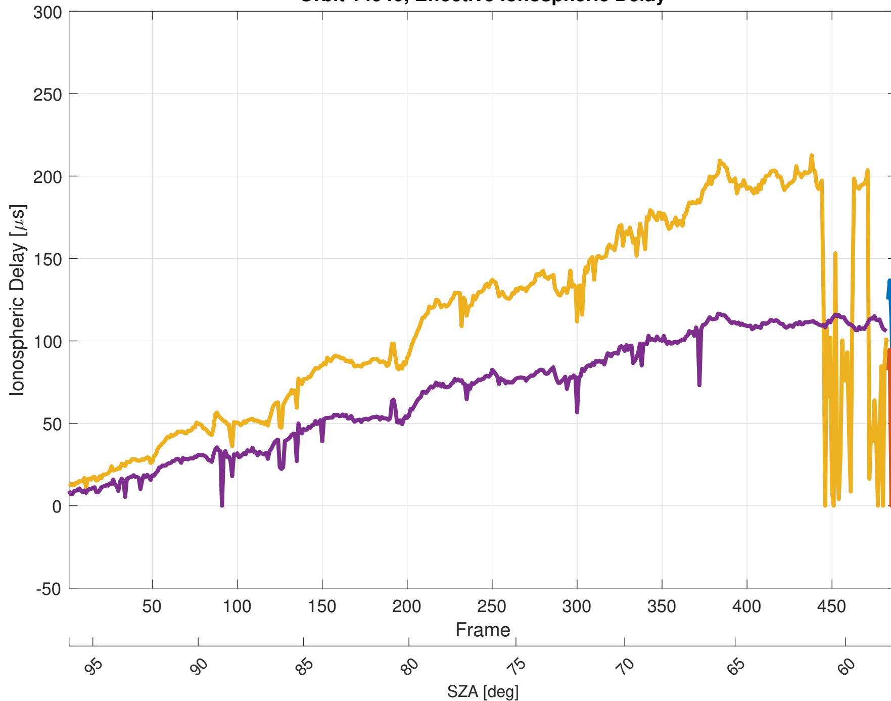
Orbit 14940, Effective Ionospheric Delay
