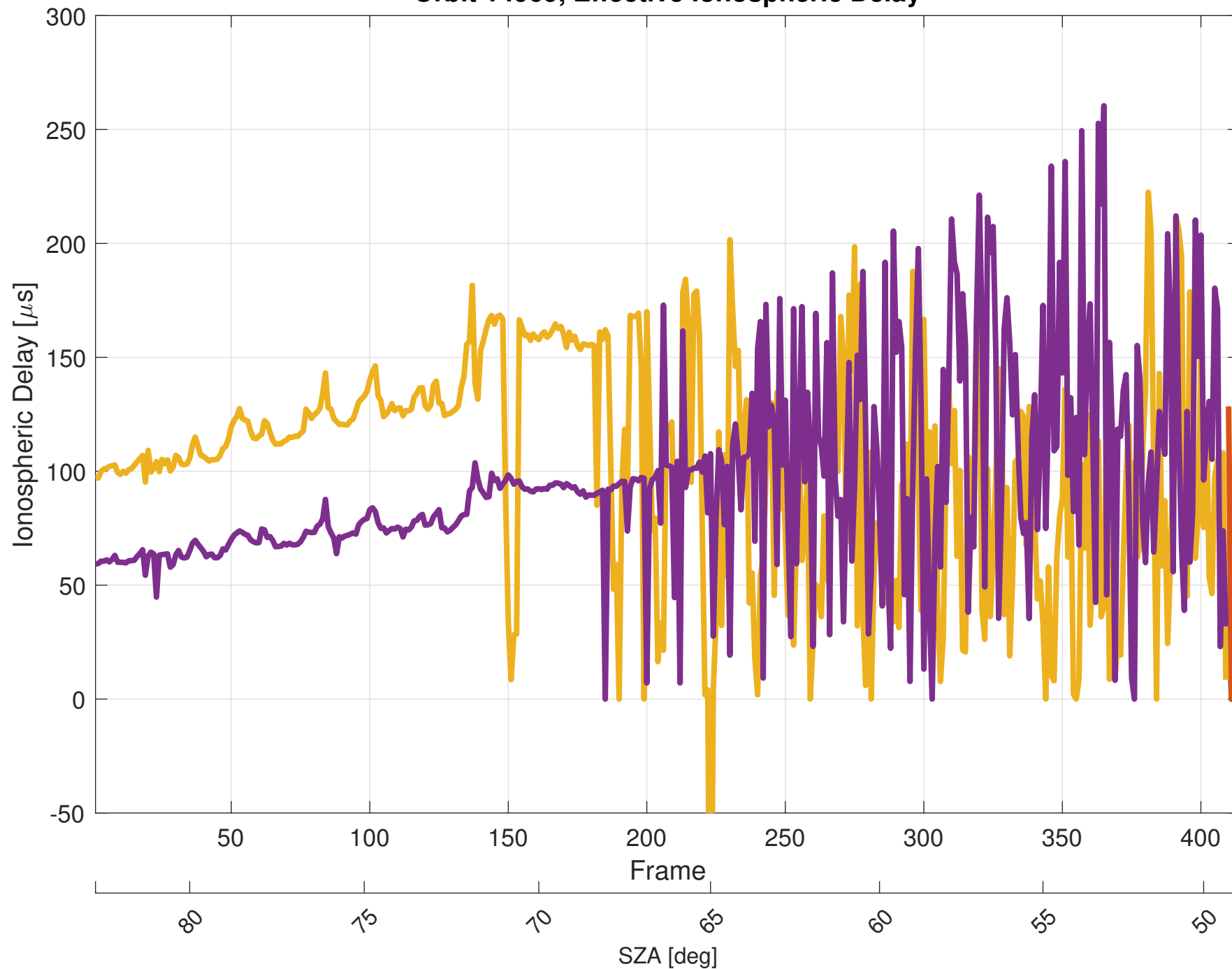
Orbit 14969, Effective Ionospheric Delay
