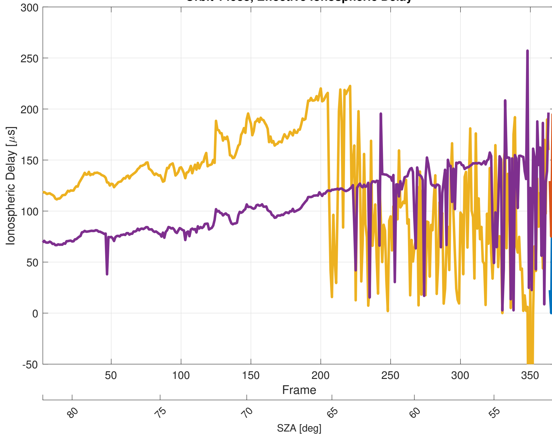
Orbit 14983, Effective Ionospheric Delay
