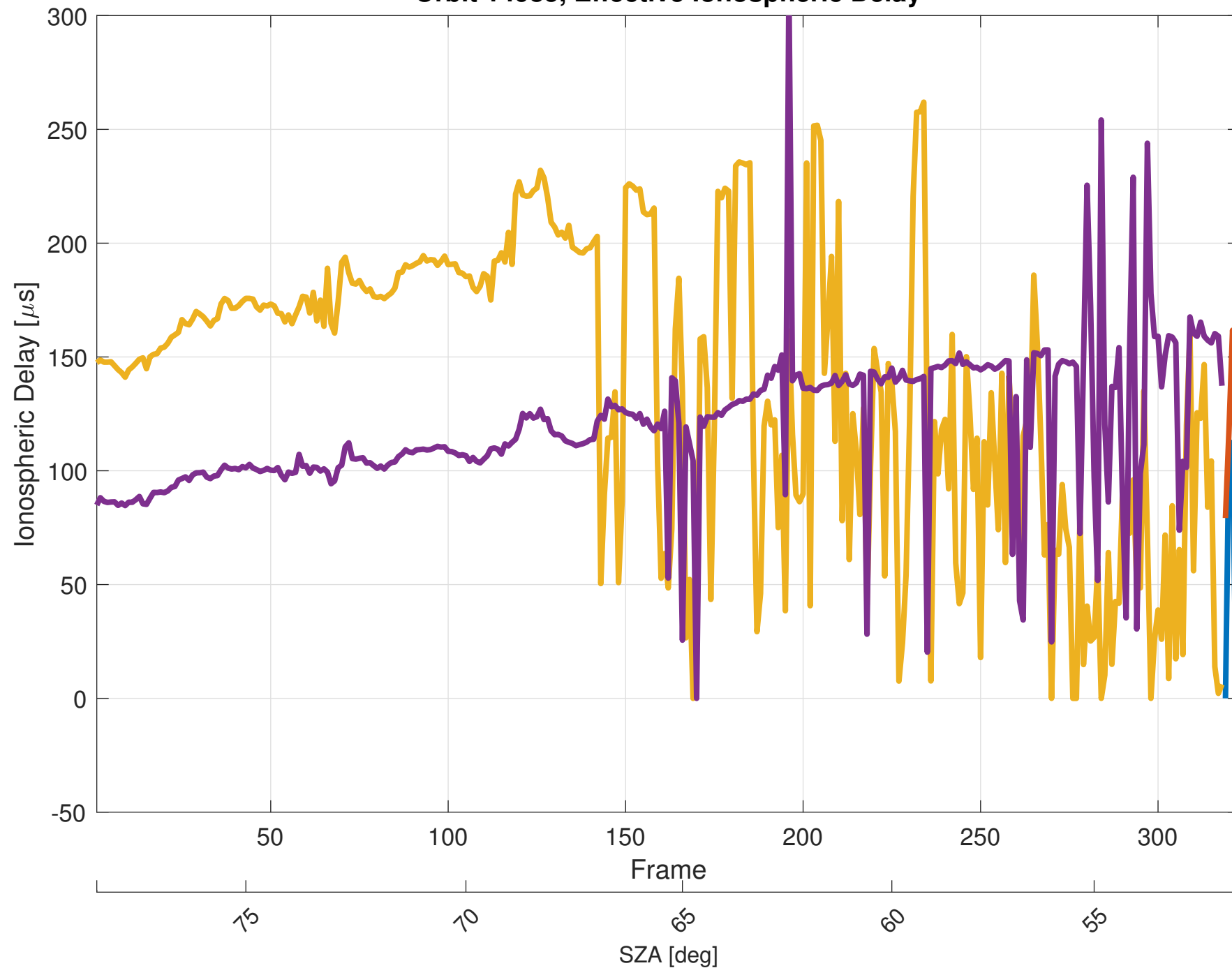
Orbit 14985, Effective Ionospheric Delay
