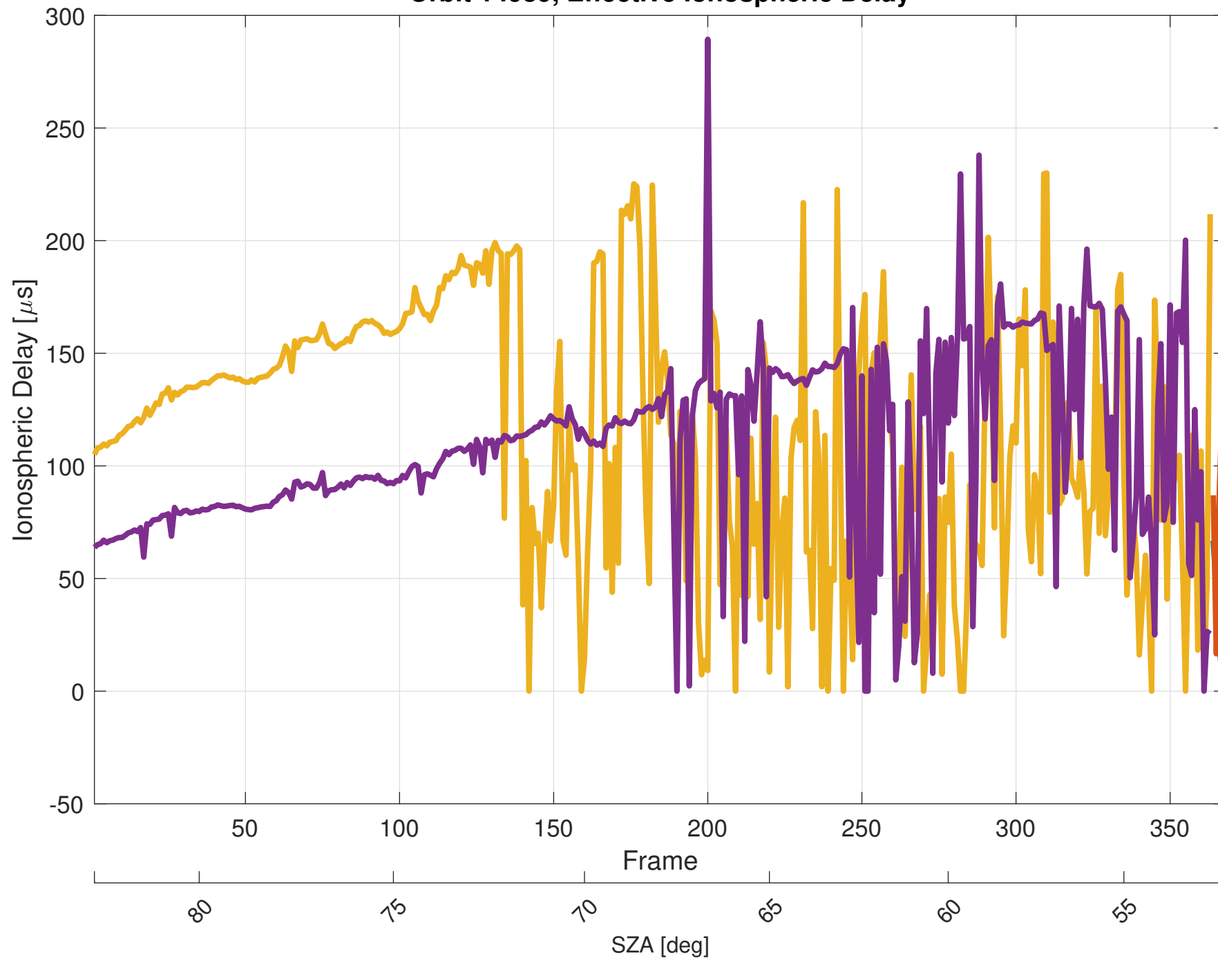
Orbit 14989, Effective Ionospheric Delay
