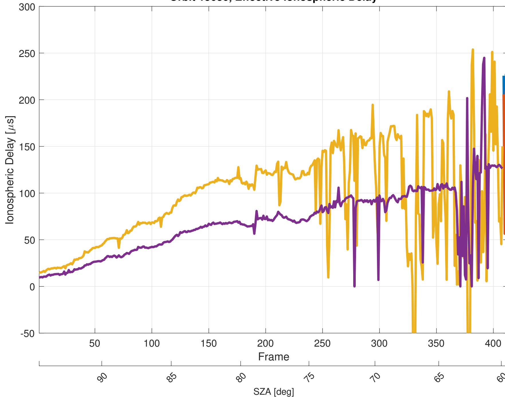
Orbit 15030, Effective Ionospheric Delay
