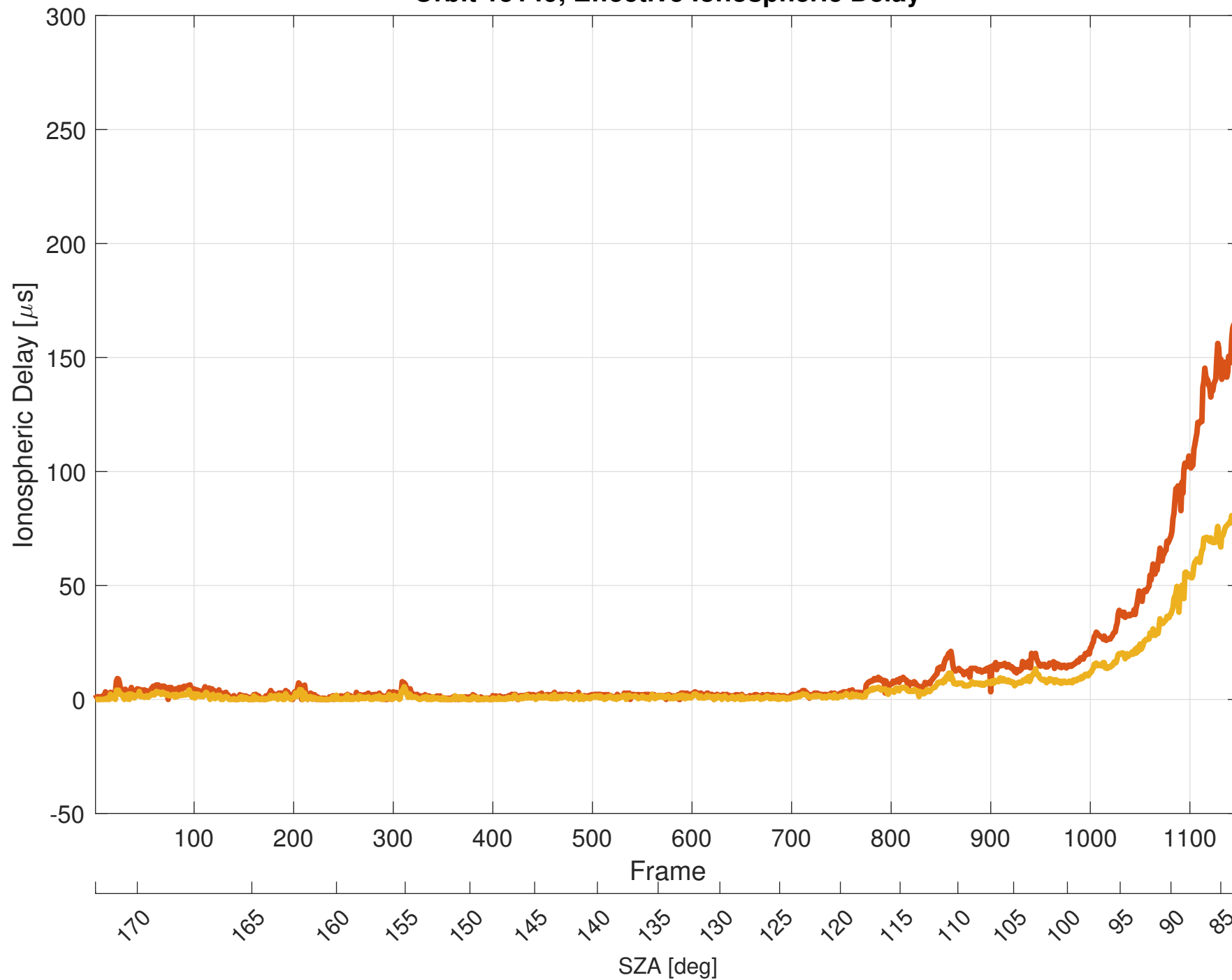
Orbit 15149, Effective Ionospheric Delay
