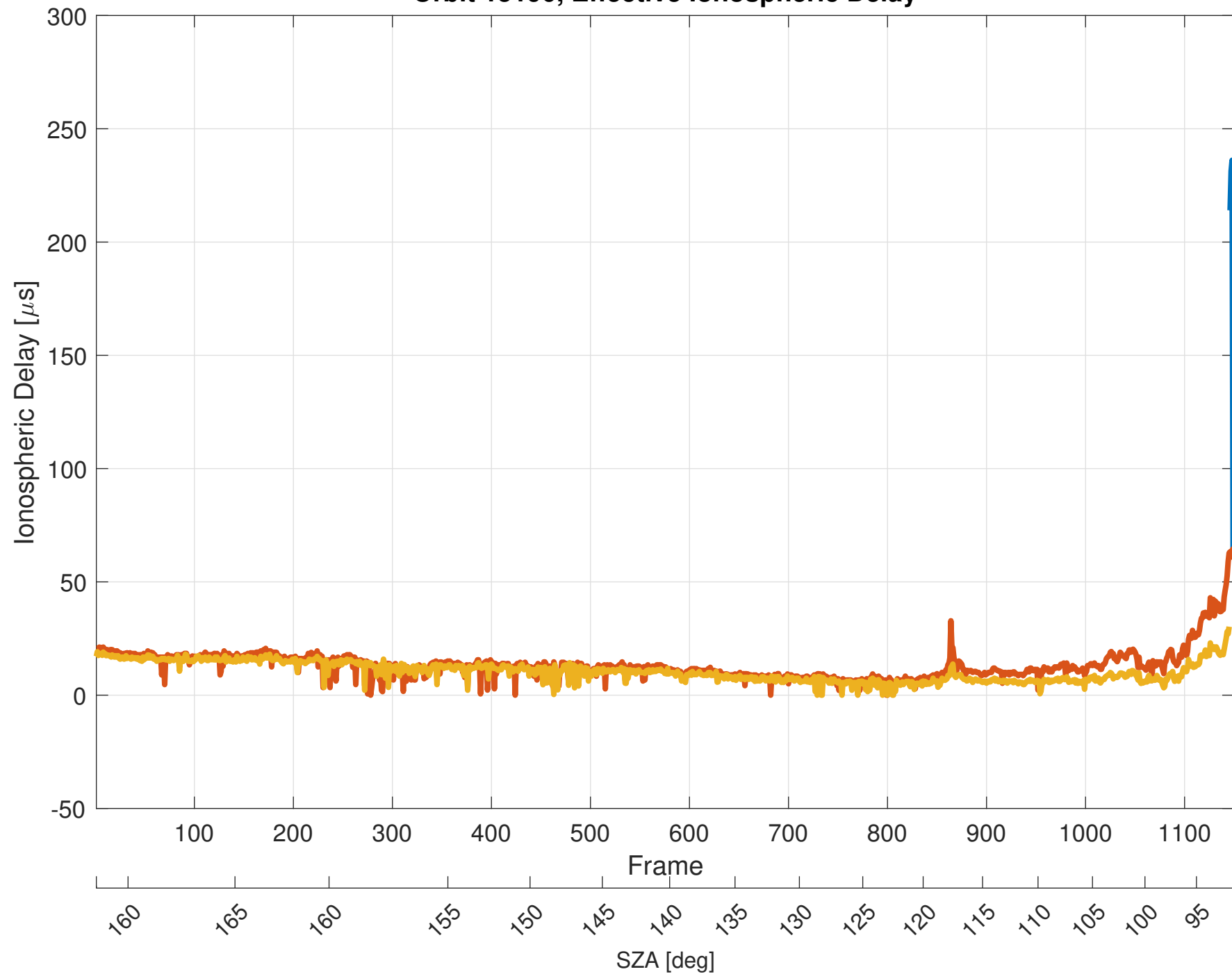
Orbit 15190, Effective Ionospheric Delay
