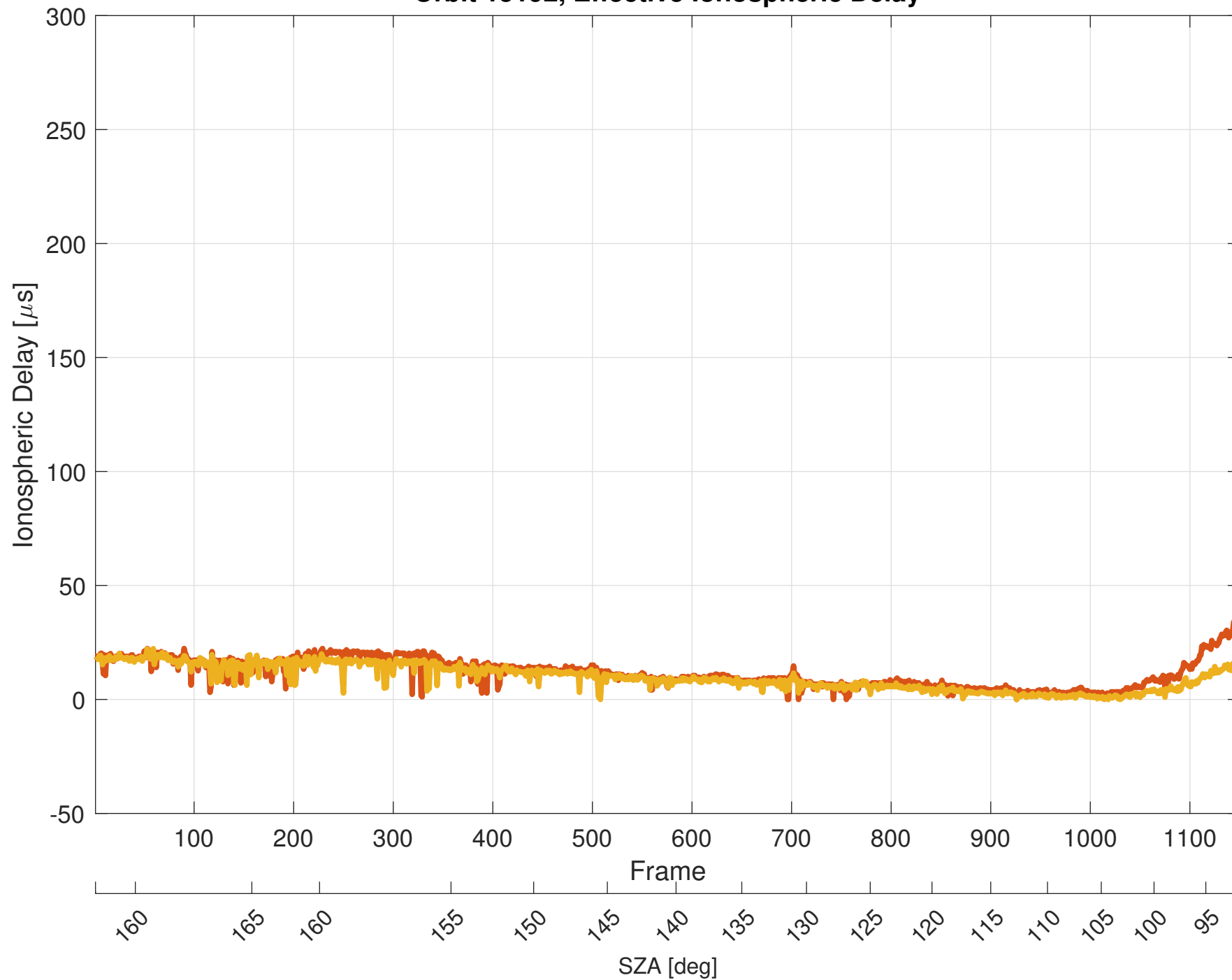
Orbit 15192, Effective Ionospheric Delay
