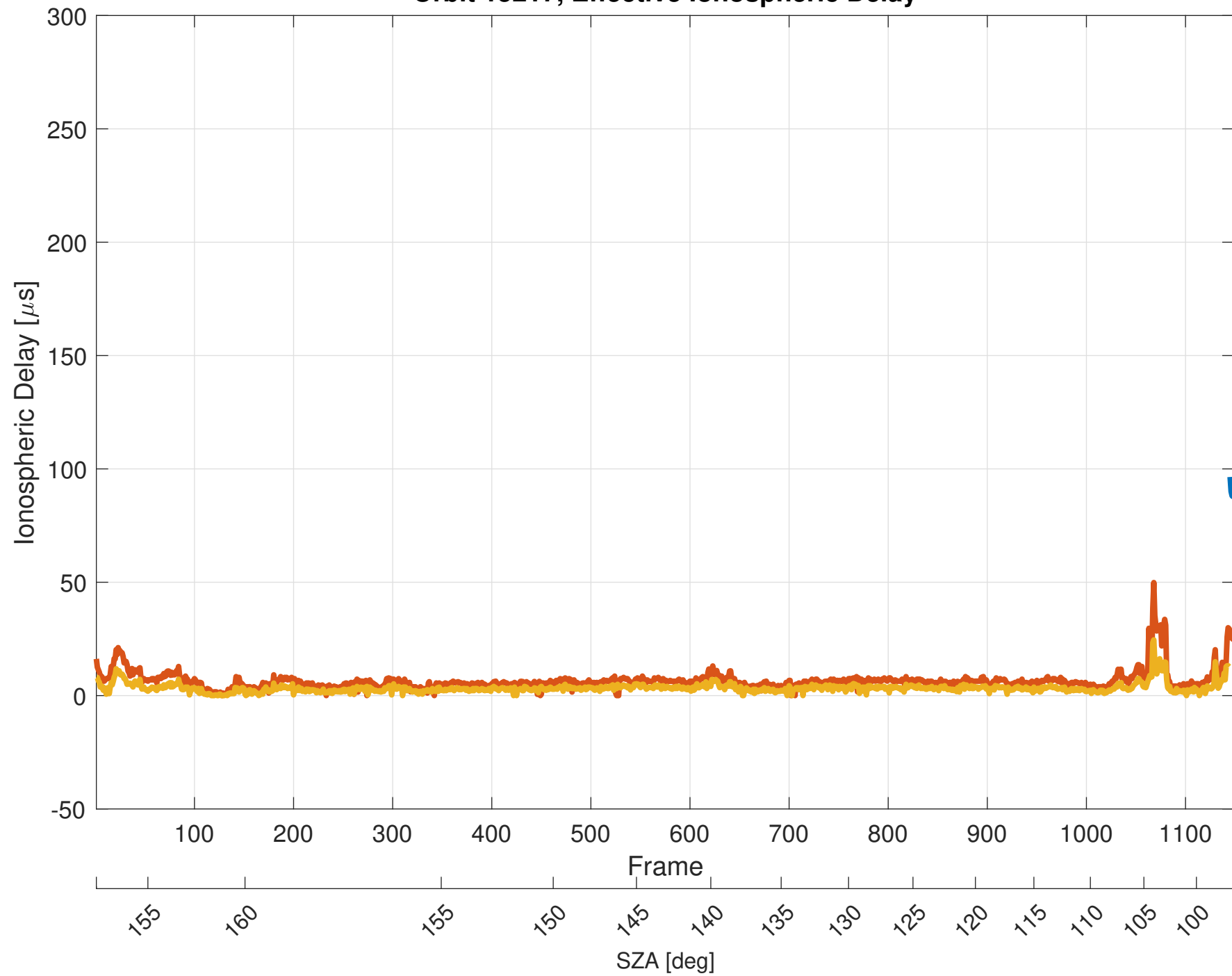
Orbit 15217, Effective Ionospheric Delay
