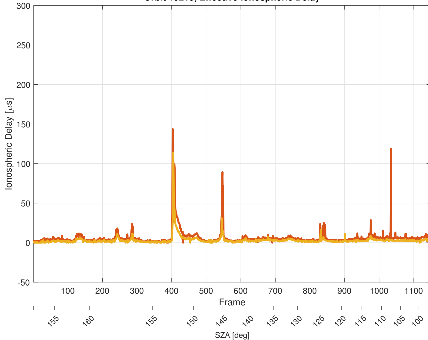
Orbit 15219, Effective Ionospheric Delay
