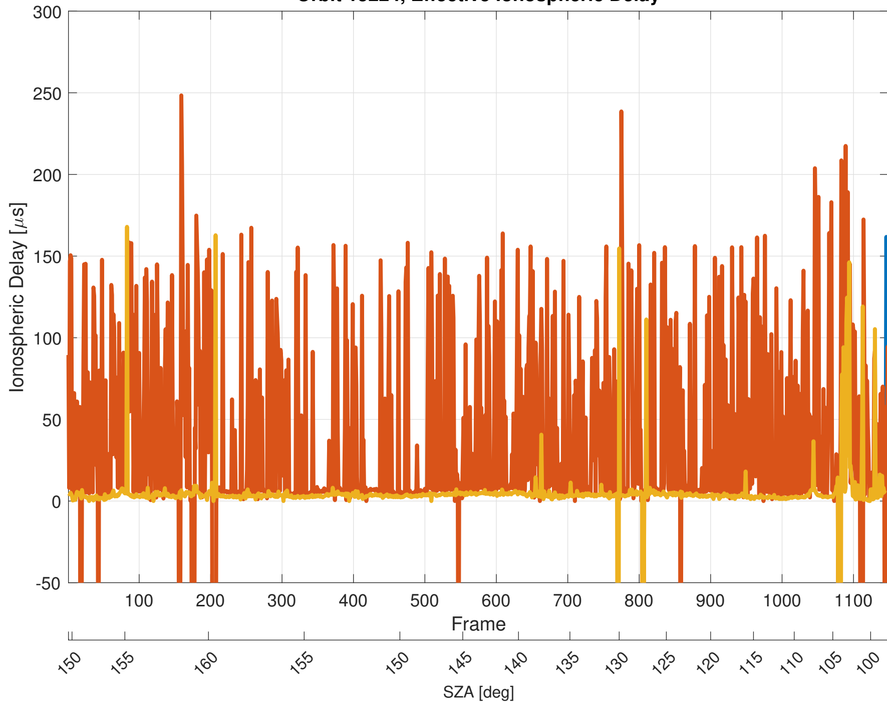
Orbit 15224, Effective Ionospheric Delay
