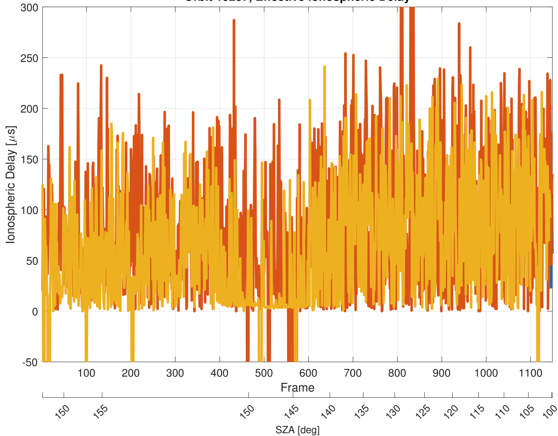
Orbit 15237, Effective Ionospheric Delay
