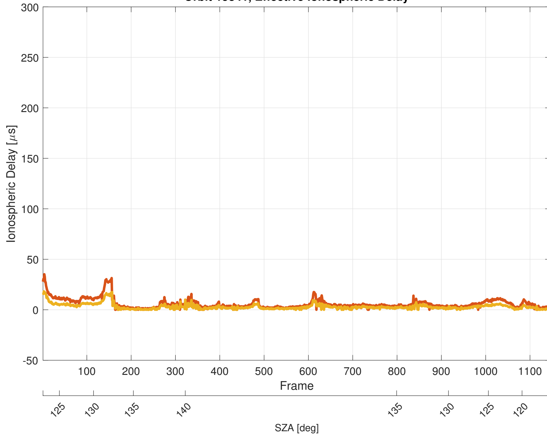
Orbit 15341, Effective Ionospheric Delay
