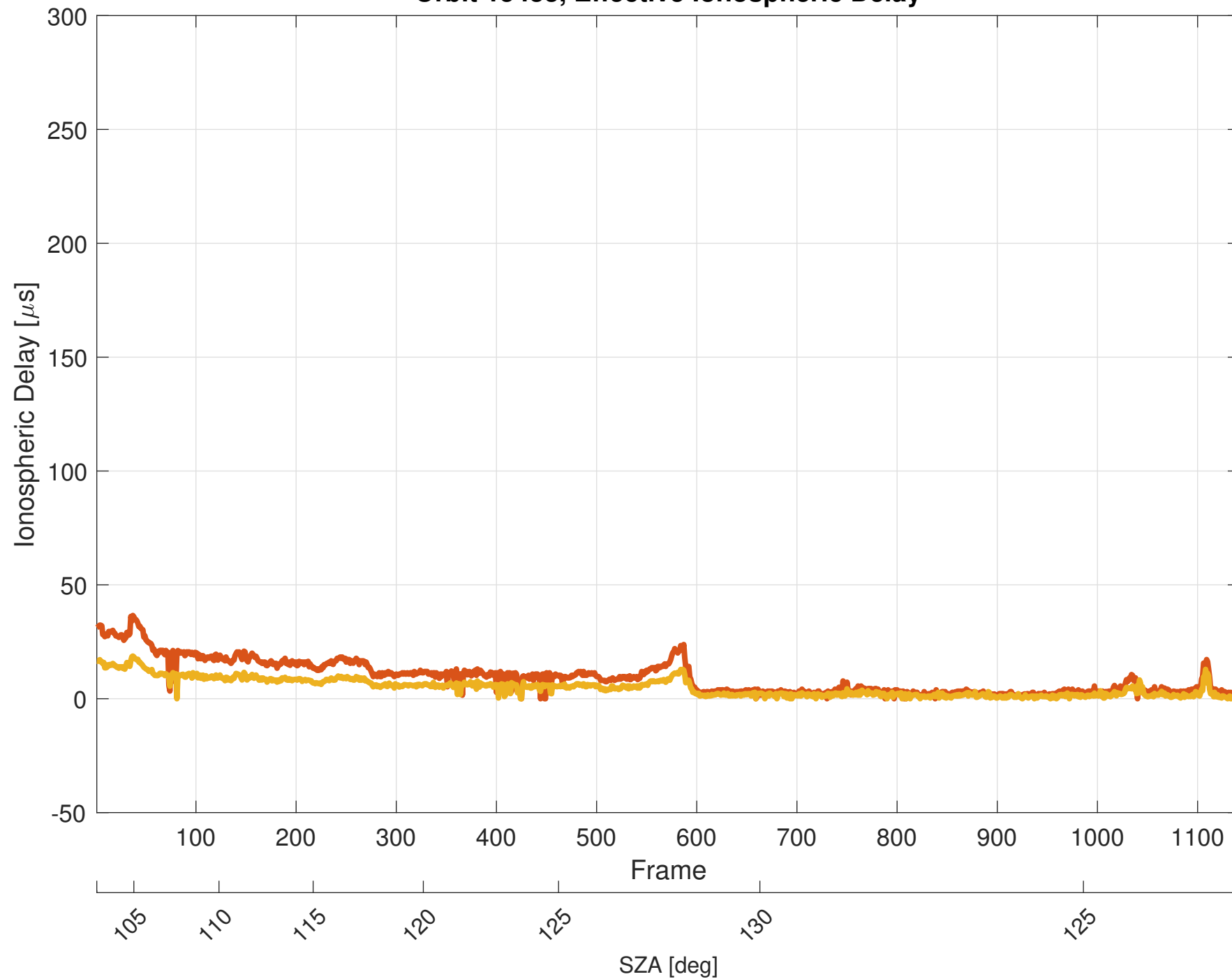
Orbit 15433, Effective Ionospheric Delay
