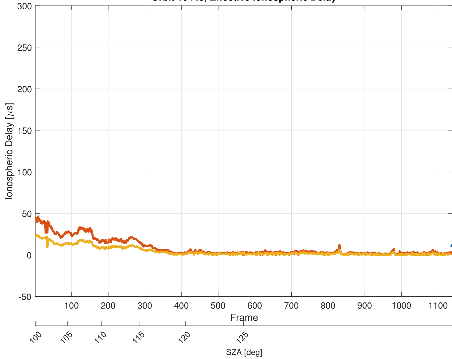
Orbit 15448, Effective Ionospheric Delay
