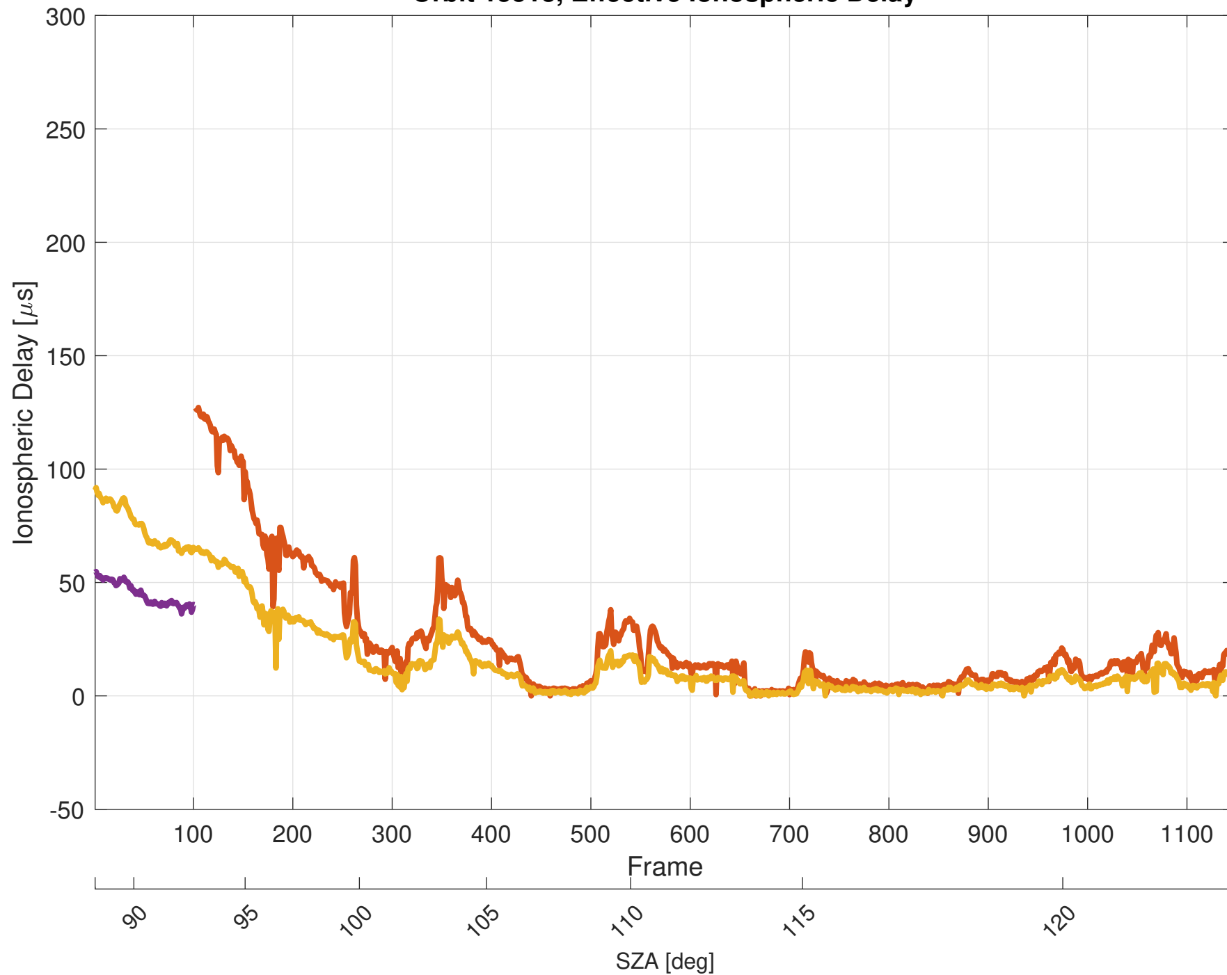
Orbit 15513, Effective Ionospheric Delay
