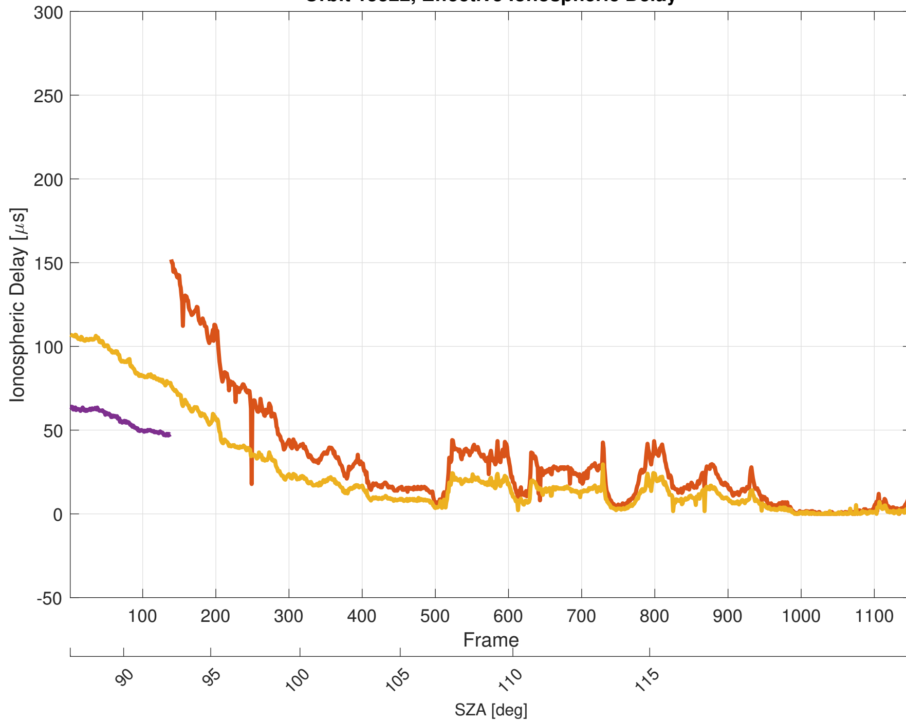
Orbit 15522, Effective Ionospheric Delay
