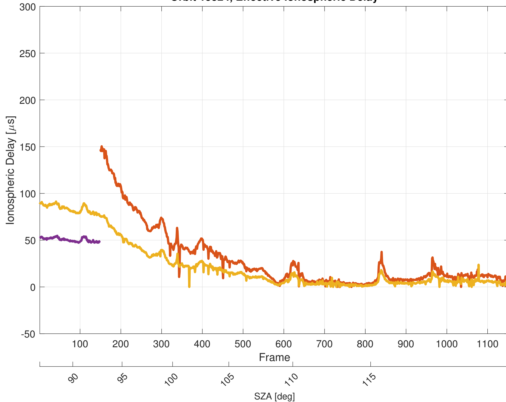
Orbit 15524, Effective Ionospheric Delay
