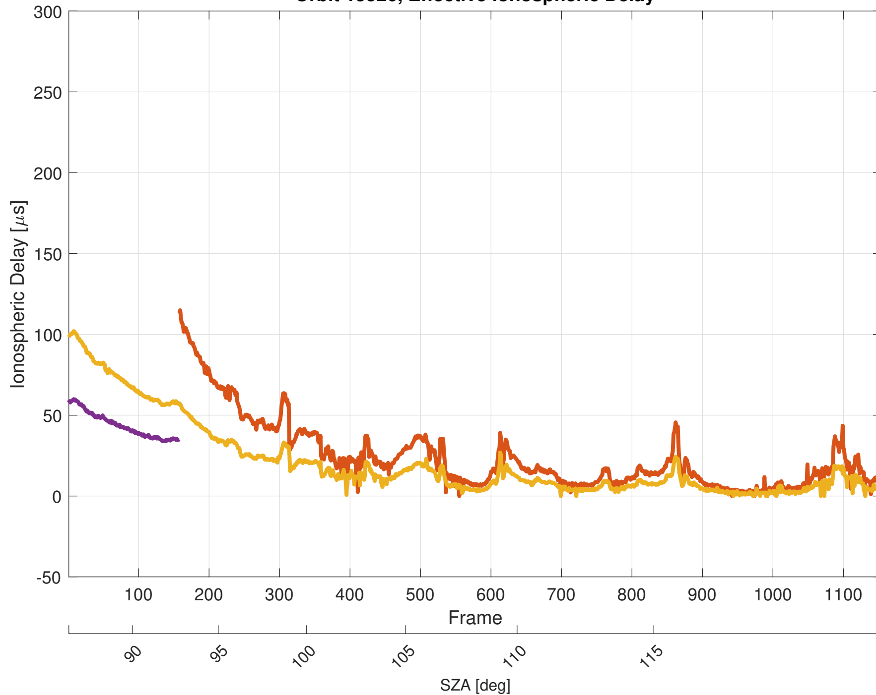
Orbit 15526, Effective Ionospheric Delay
