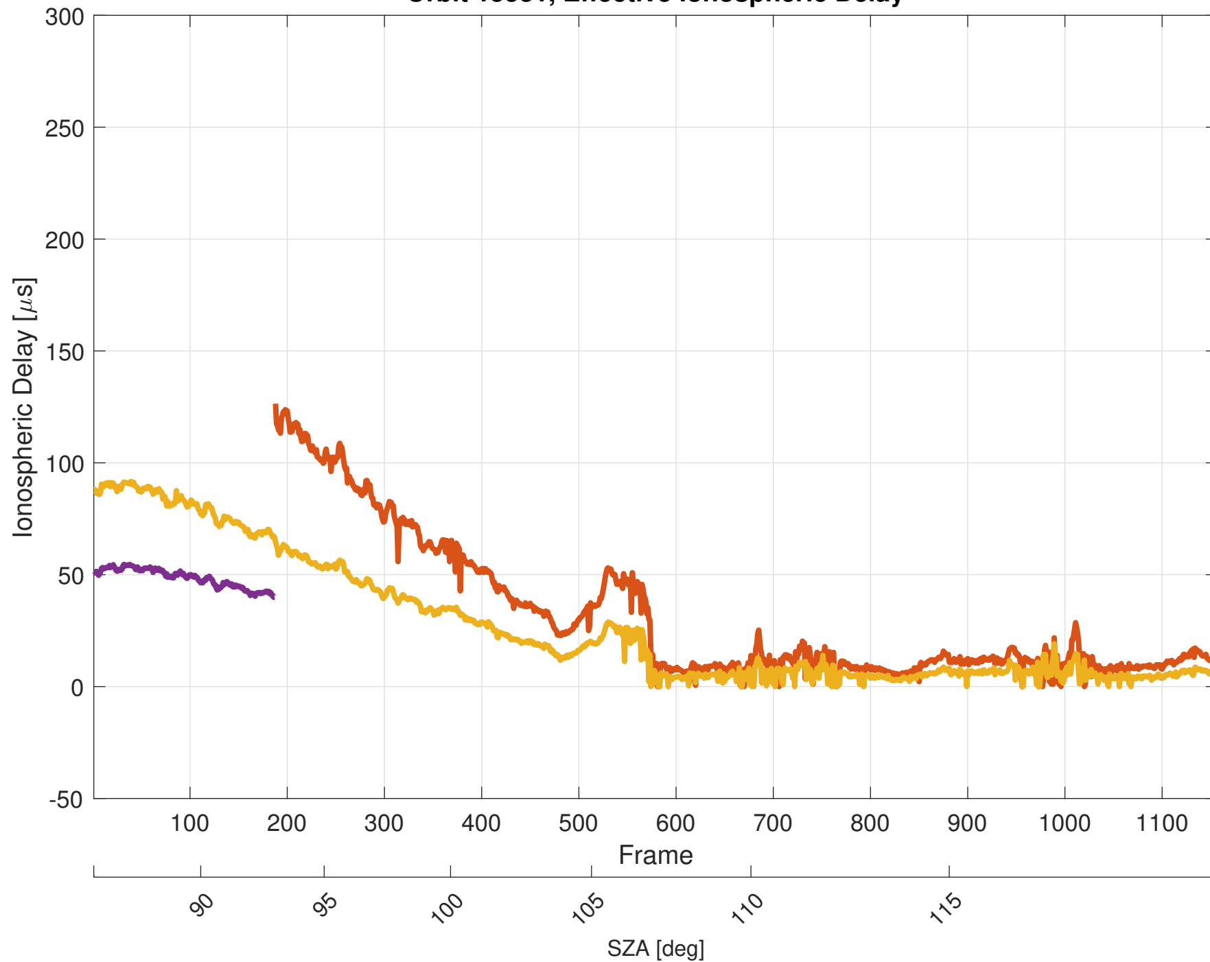
Orbit 15531, Effective Ionospheric Delay
