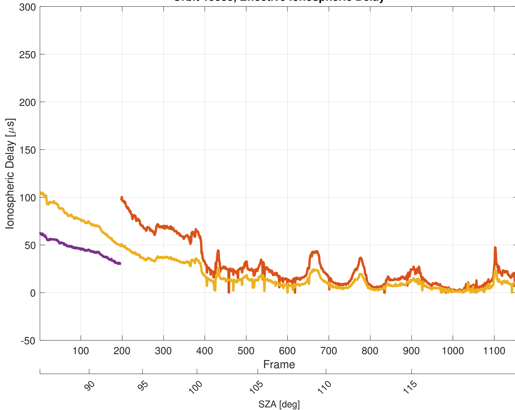
Orbit 15533, Effective Ionospheric Delay
