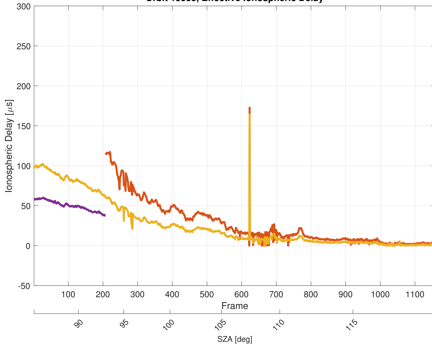
Orbit 15535, Effective Ionospheric Delay
