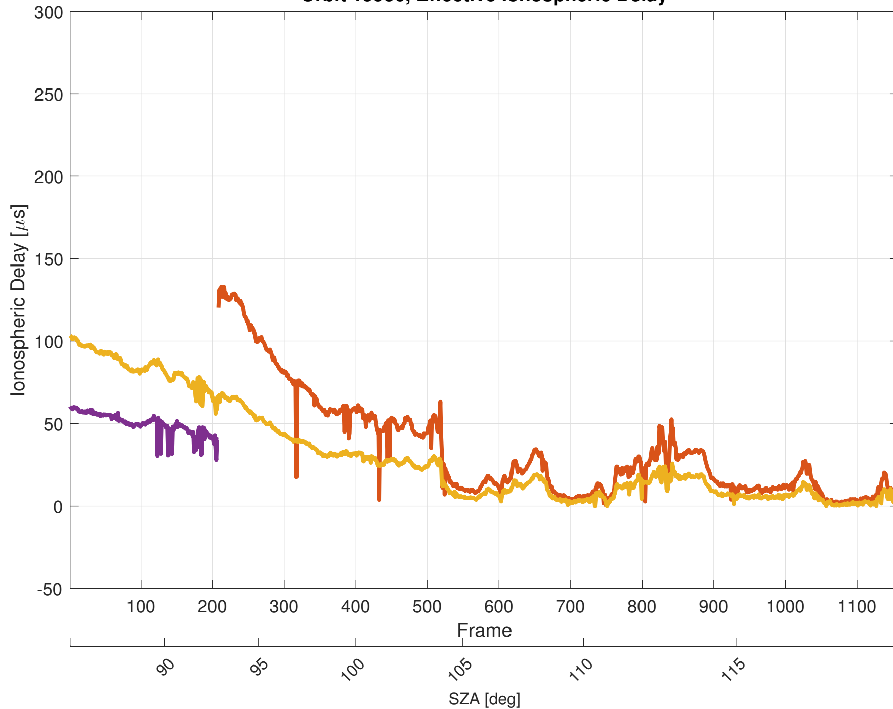
Orbit 15536, Effective Ionospheric Delay
