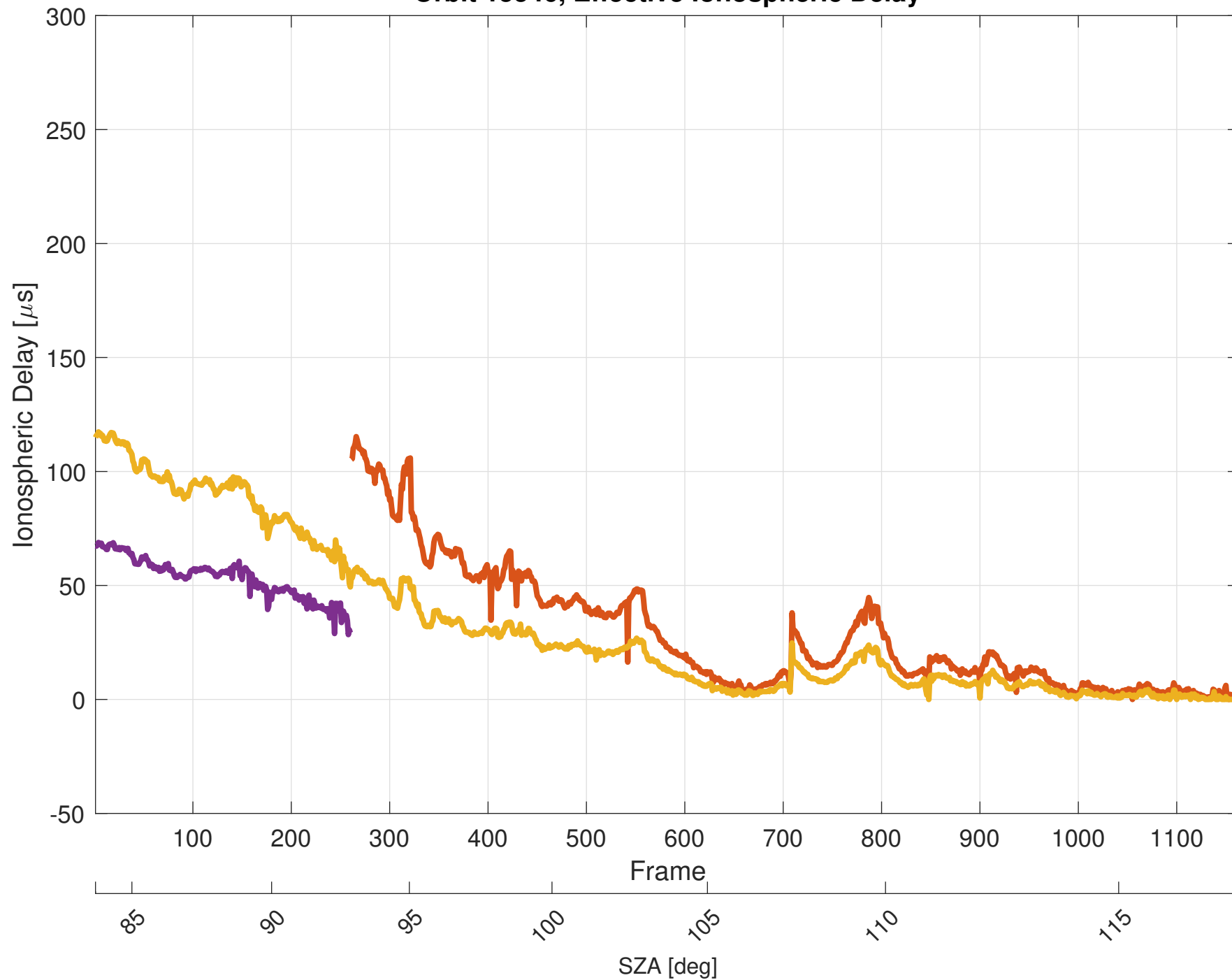
Orbit 15546, Effective Ionospheric Delay
