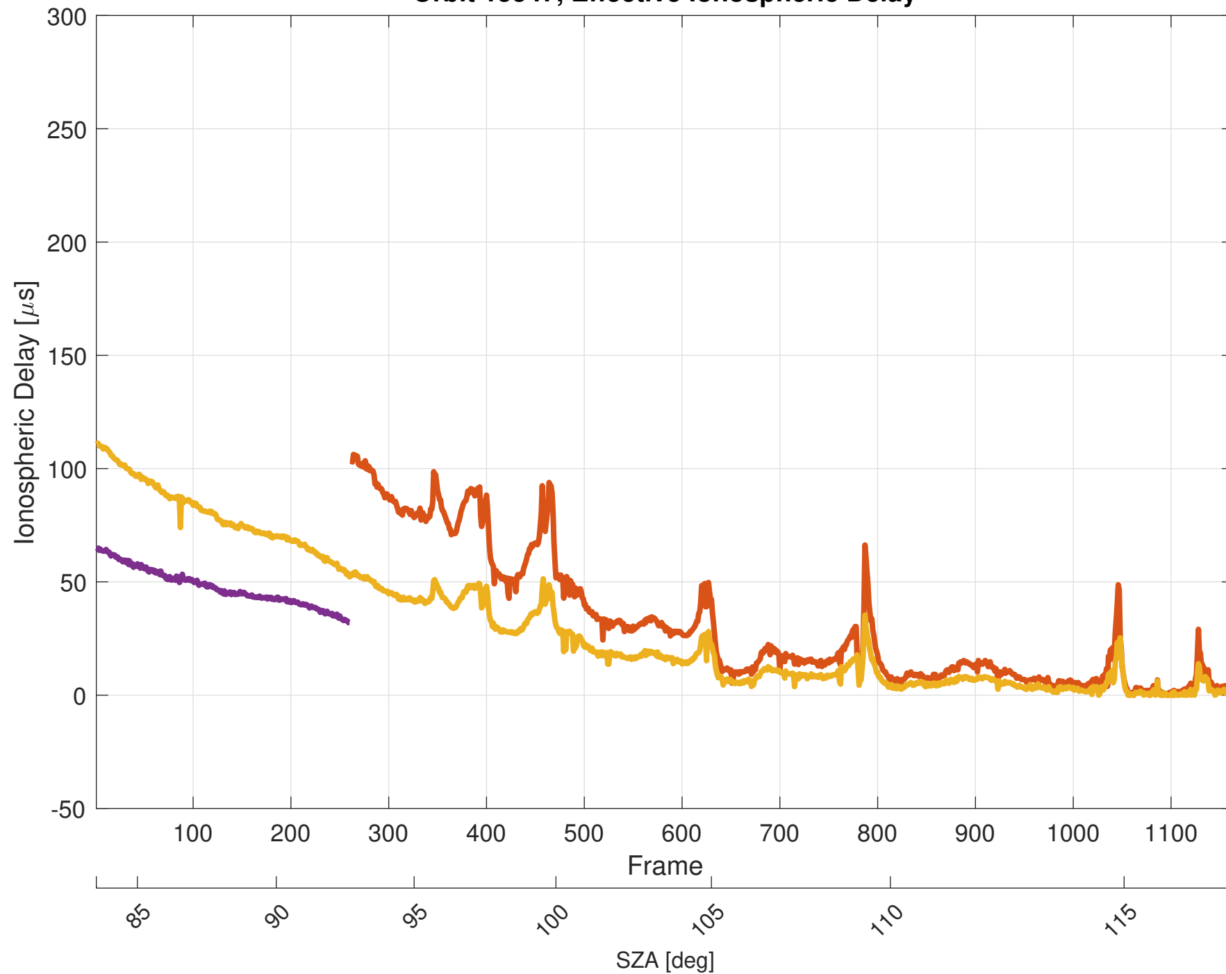
Orbit 15547, Effective Ionospheric Delay
