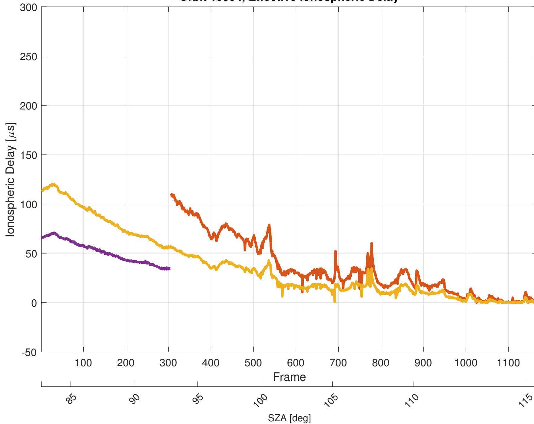
Orbit 15554, Effective Ionospheric Delay
